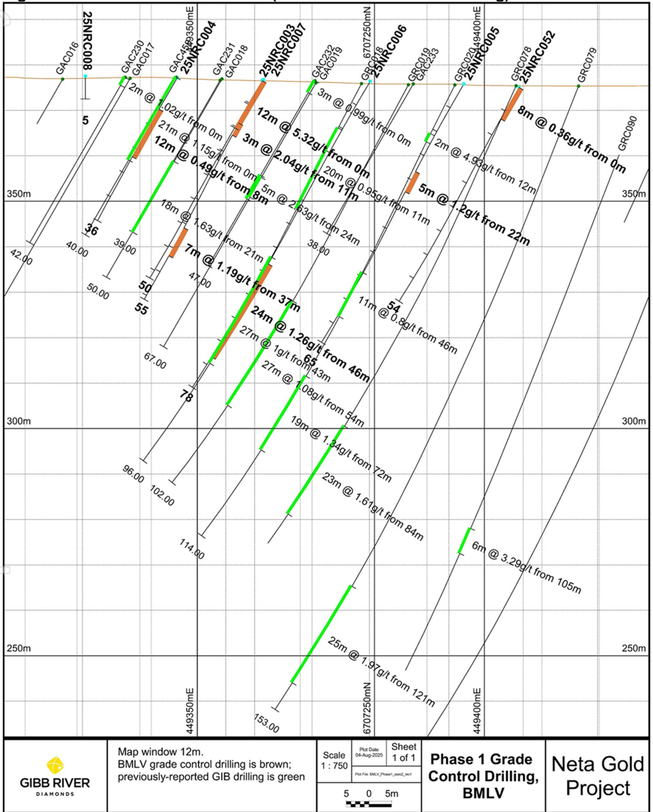
Figure 3: Neta Cross Section A – A' (Phase 1 Grade Control Drilling)
