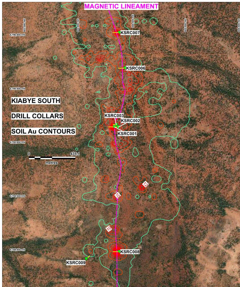
Figure 4: Location of RC drilling at Kiabye South. The location of the magnetic lineament is shown as the magenta dashed line and gold-in-soil contours (ppb) are shown in red. Six of the holes lie along the Kiabye South magnetic lineament target, while KSRC009 was designed to test for mineralisation associated with gossan sample KPR065.
