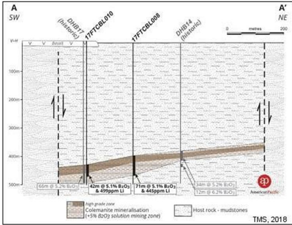
Figure 7.1: Cross-section through the Fort Cady deposit
