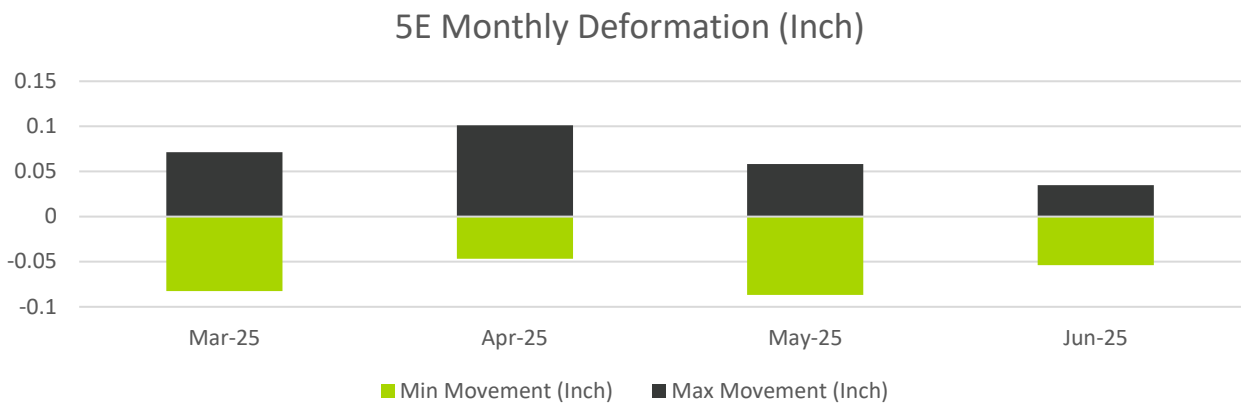
Figure 13.6: Micro-deformation results
