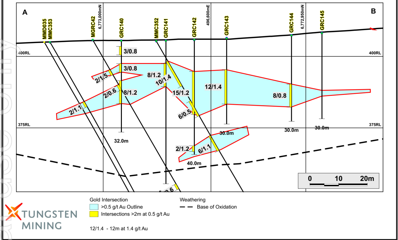
Figure 3. Section A-B showing horizontal supergene gold mineralisation at the Mulgine Trench.
