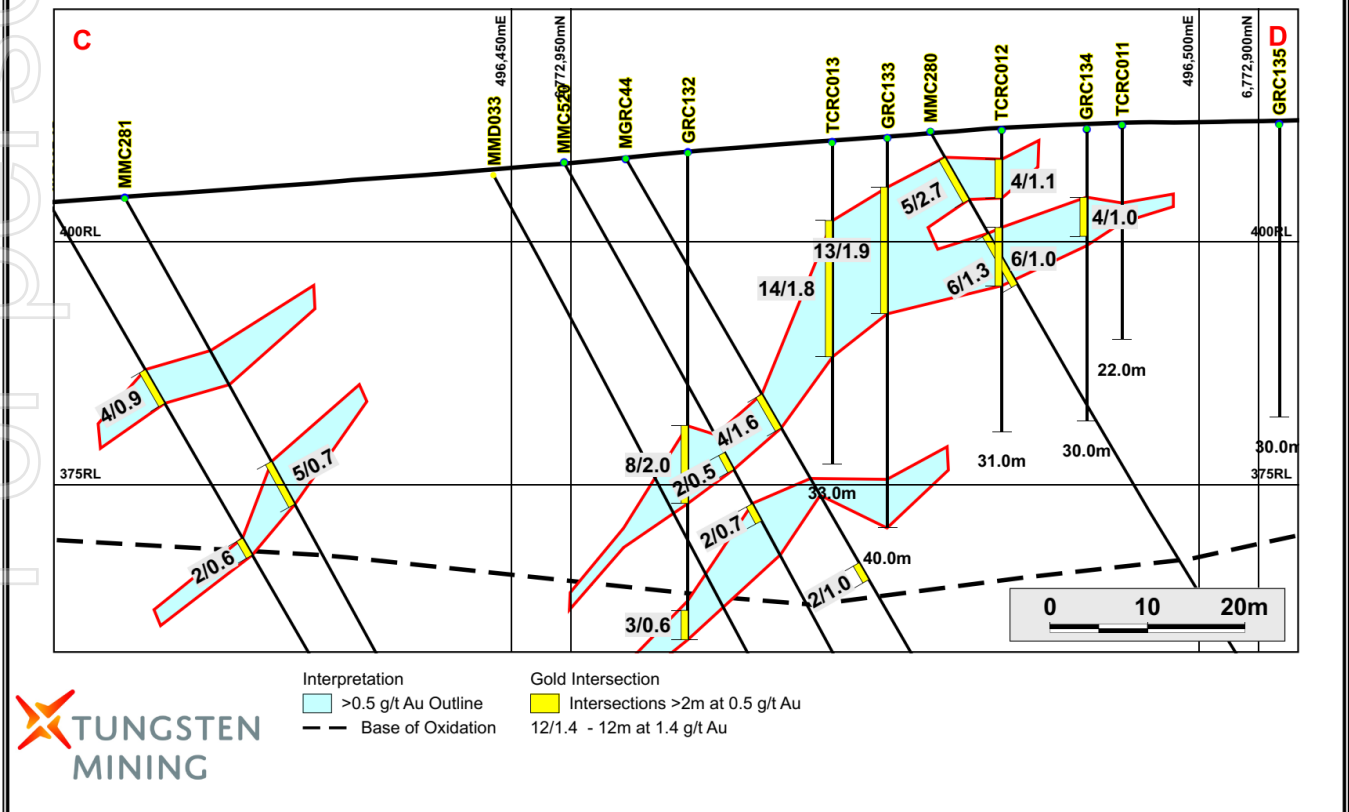
Figure 4. Section C-D showing structurally controlled northwest dipping zones gold mineralisation at the Mulgine Trench.
