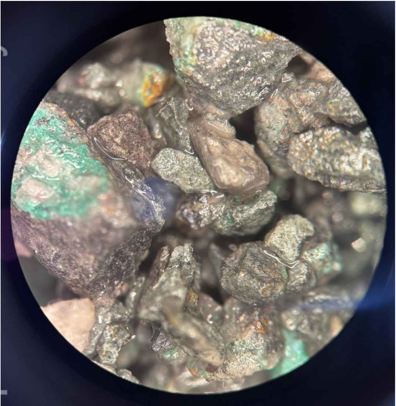
Figure 3 - Example of chalcocite and malachite rich RC drill chips from 15.24m to 16.76m in DAN25019. Cautionary Statement: The Company cautions that, with respect to any visual mineralisation indicators, visual observations and estimates of mineral abundance and uncertain in nature and should not be taken as a substitute or proxy for appropriate laboratory analysis. Visual estimates also potentially provide no information regarding impurities or deleterious physical properties relevant to valuations. Assay results from the drilling and sampling programmes will be required to understand the grade and extent of mineralisation. Initial assay results are expected in the September quarter.
