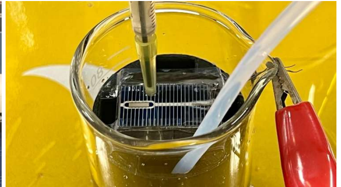
Figure 2 – Jet Electrochemical Silver Extraction Probe
