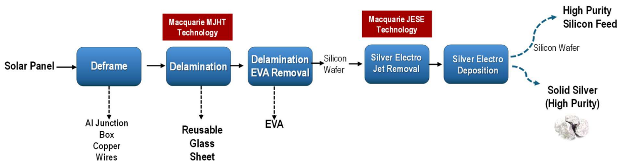
Figure 9 – Incorporation of MQU MJHT and JESE Technology in Silver Extraction Process
