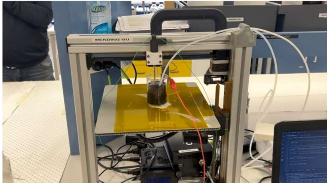
Figure 2 – Jet Electrochemical Silver Extraction Probe
