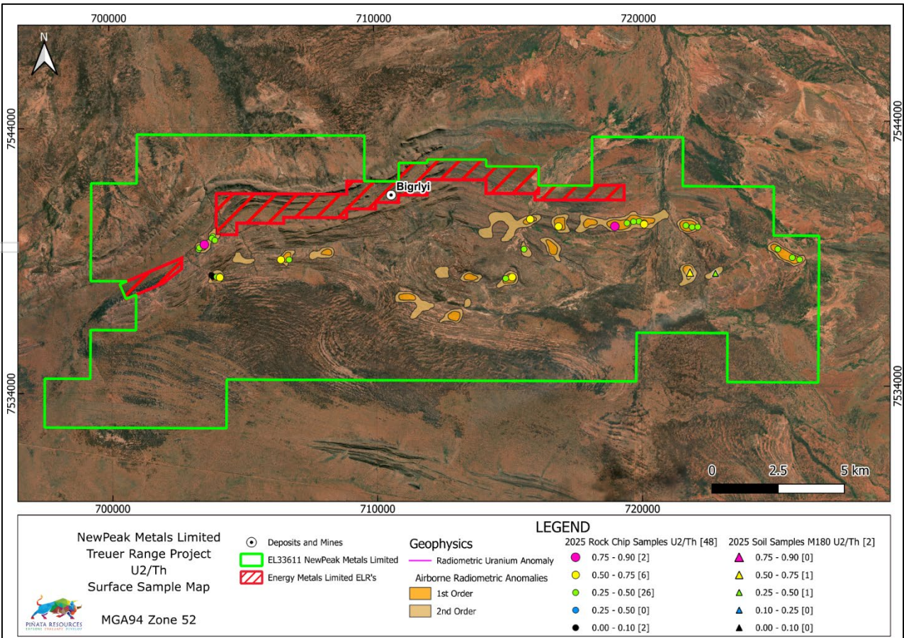
Figure 14: Uranium Squared / Thorium (U²/Th) for Rock Chip samples and Soil Samples (sieved minus 180µm fraction) for the Treuer Range Project
