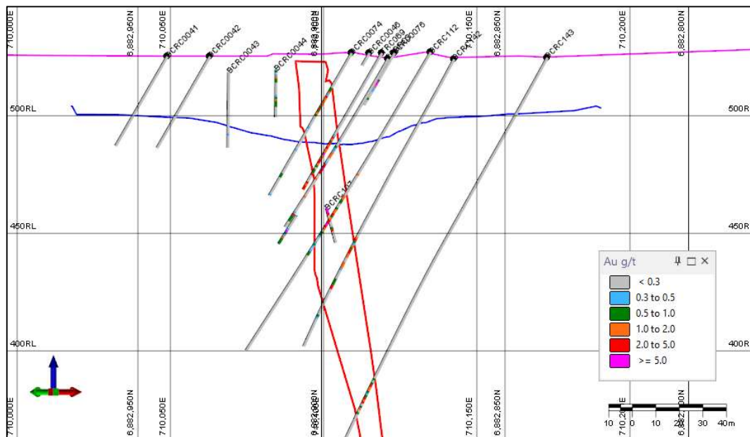
Figure 4. Bellchambers Cross Section Interpretation
