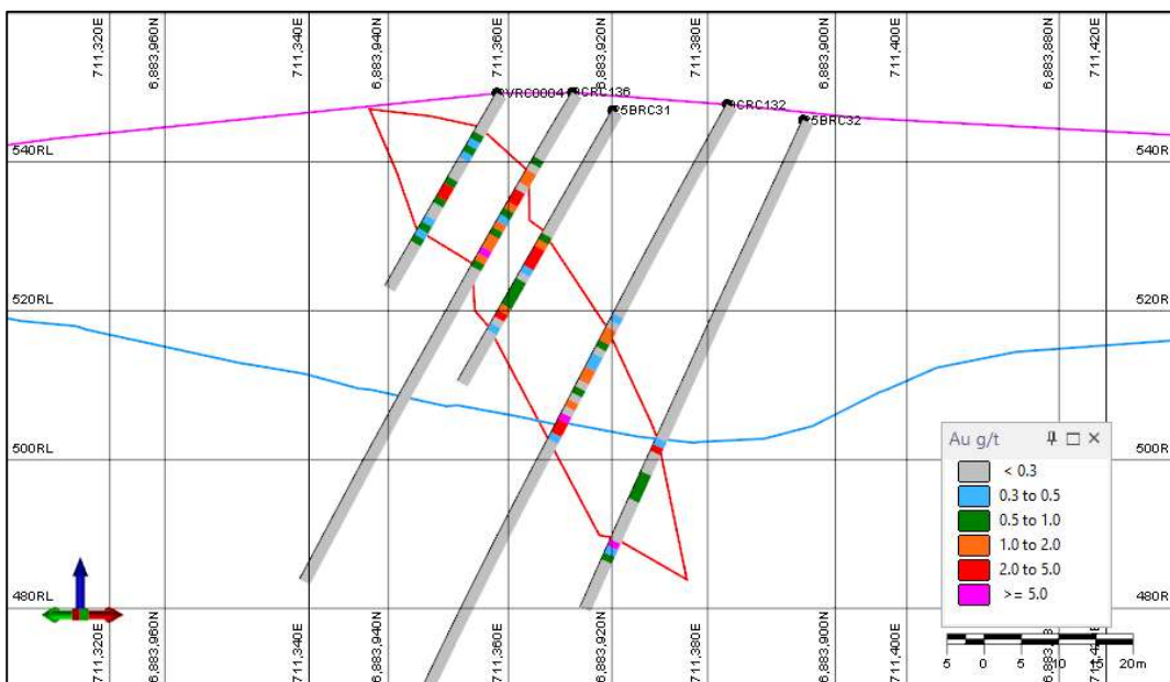
Figure 5. Range View Cross Section Interpretation
