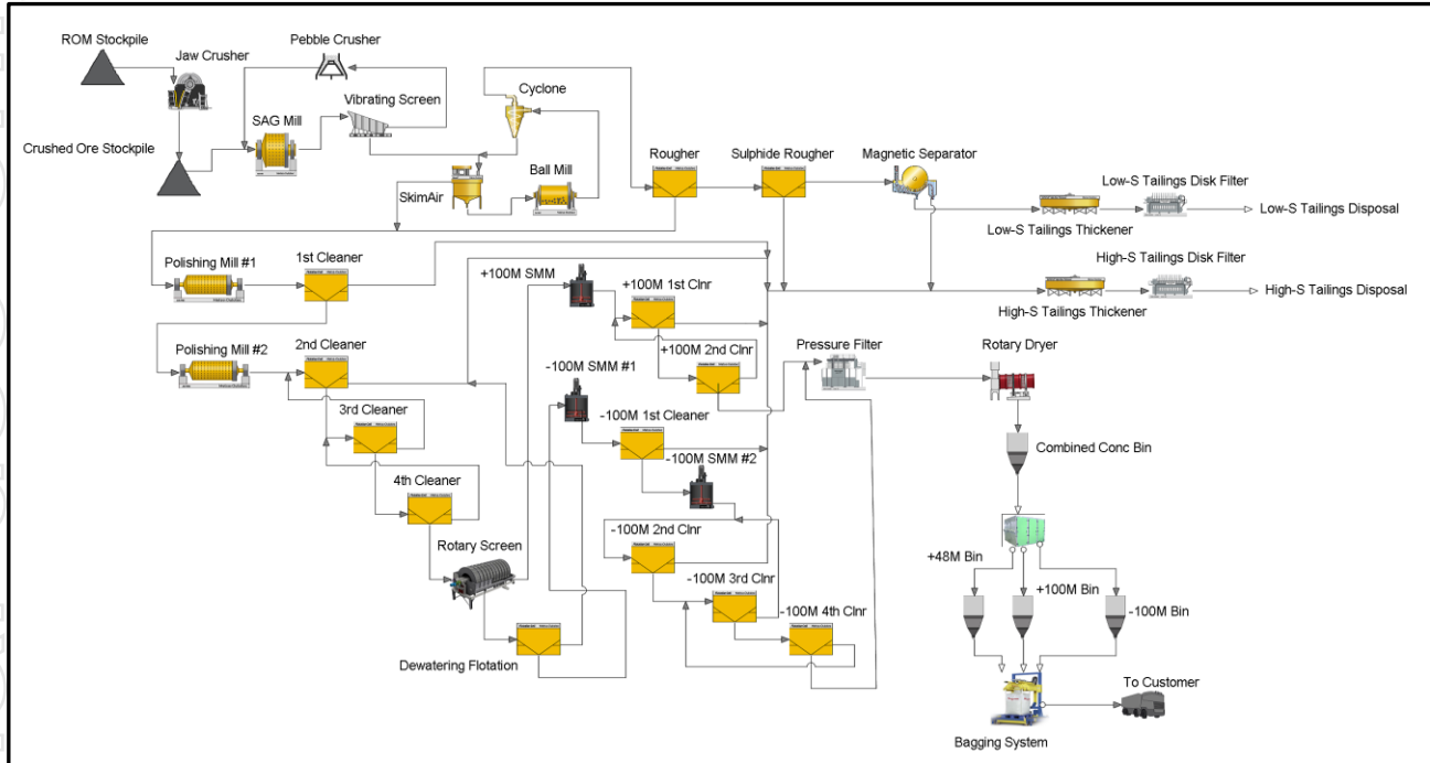
Figure 10: Lac Carheil Graphite Project – Flake Graphite Concentrate Plant Flowsheet
