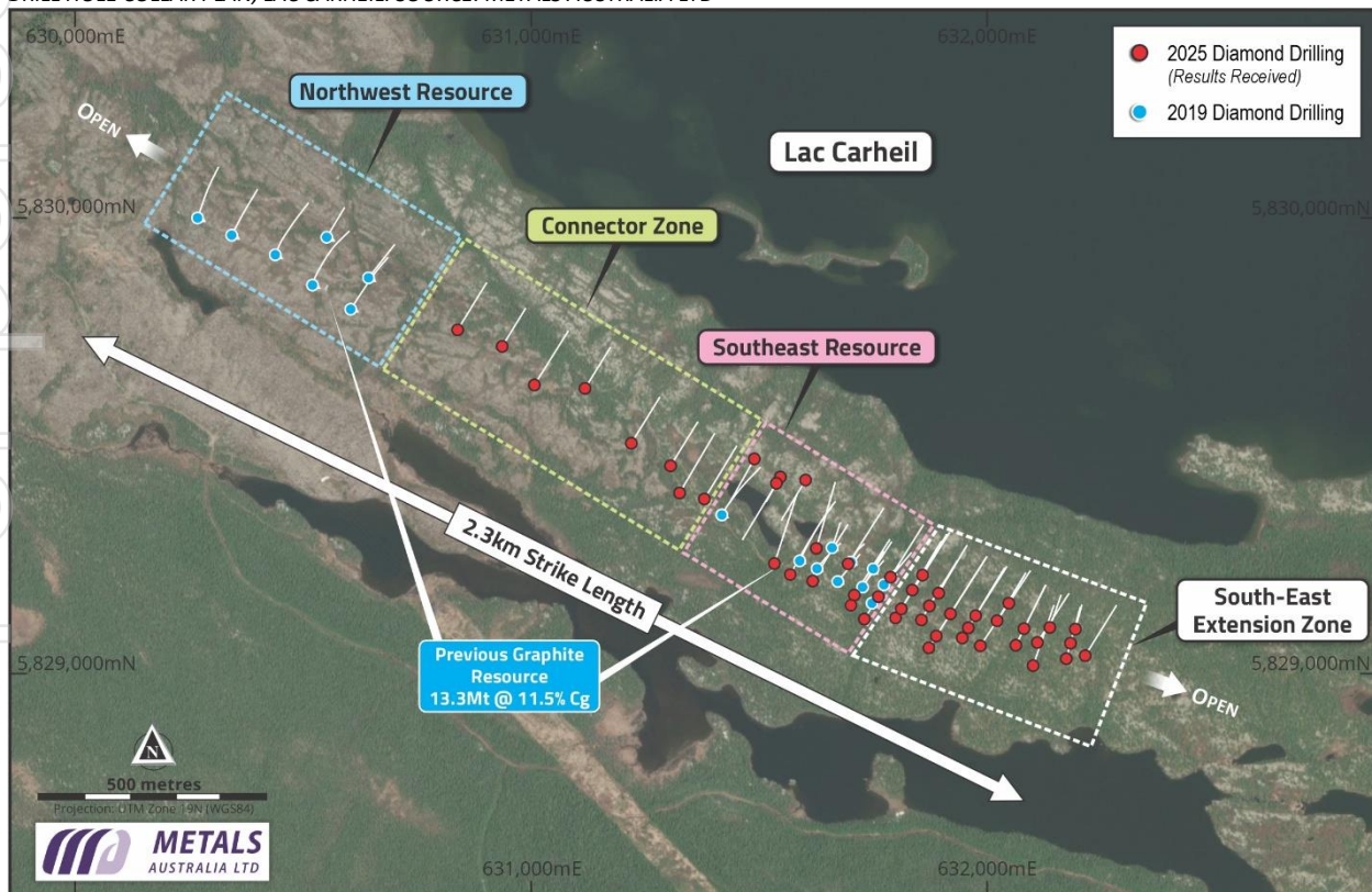
DRILL HOLE COLLAR PLAN, LAC CARHEIL. SOURCE: METALS AUSTRALIA LTD
