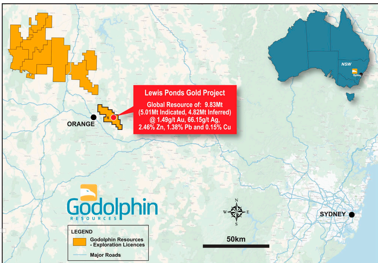
Figure 5: Location Map of Godolpin Resources Gold and Copper Projects in the Lachlan Fold Belt, NSW.
