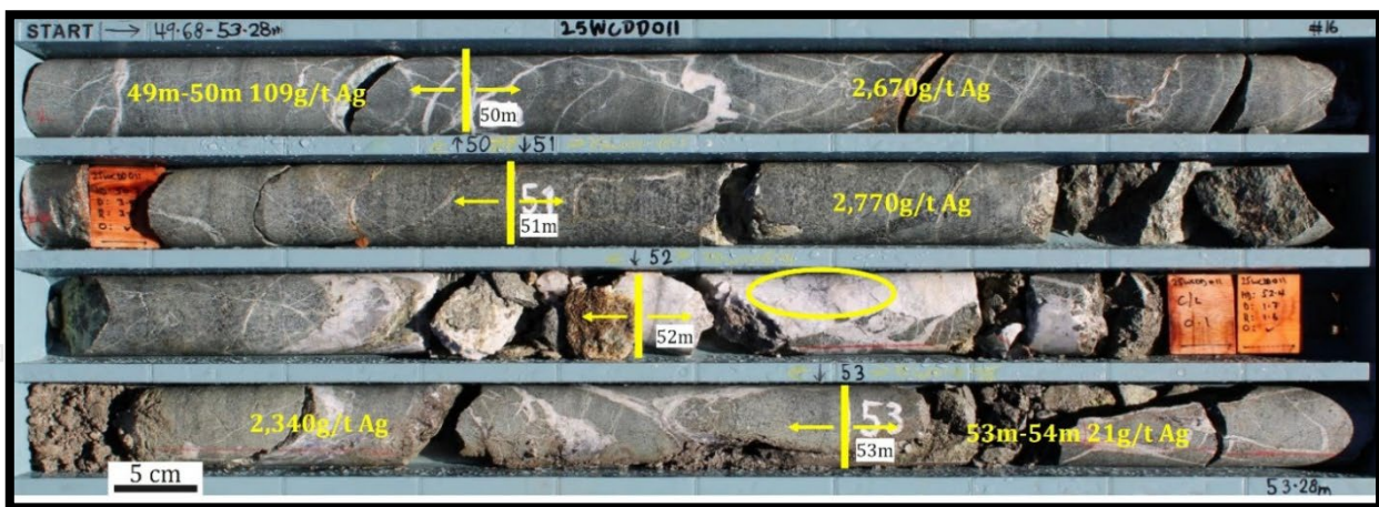
Figure 7. 25WCDD011 - visible native silver and silver sulphide minerals (yellow circle) in coarse crystalline calcite-quartz vein; The vein is hosted in fine to medium grained pyroxenite; The silver minerals are between 7mm and 8mm in size and comprise about 7% of the 86cm calcite-quartz vein commencing at 49.68m
