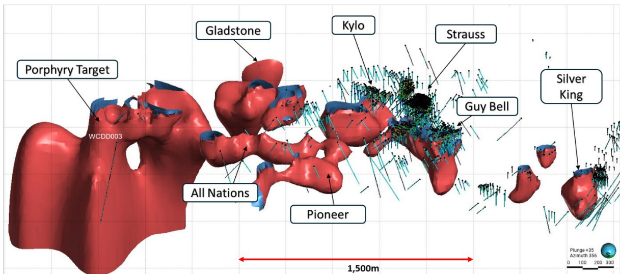
Figure 7. Isosurfaces (Chg3D 12) of chargeability and survey line locations over the Mt Carrington area.
