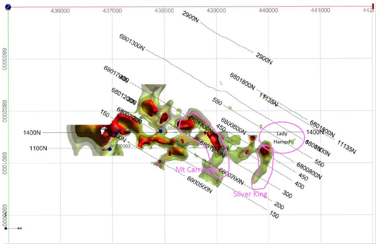
Figure 7. Isosurfaces (Chg3D 12) of chargeability and survey line locations over the Mt Carrington area.
