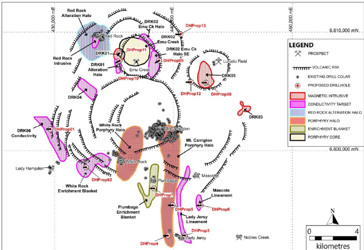
Figure 2. Interpreted Mobile-MT targets and major trends with new interpretation of nested caldera setting.
