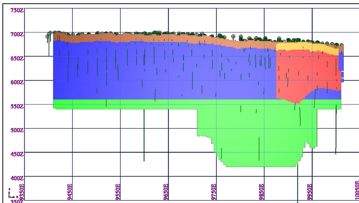
Figure 9: Block Model Sub-Domaining
