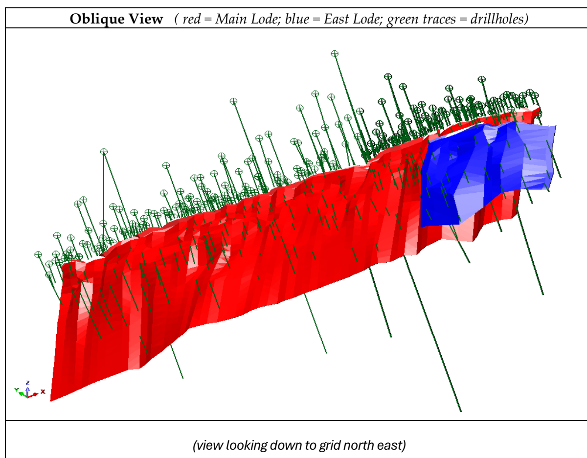
Figure 7: Granite Castle Mineral Lode Interpretation
