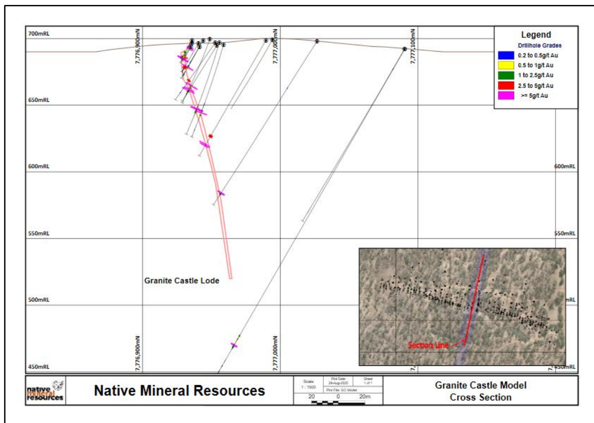
Figure 5: Schematic Cross Section for Granite Castle
