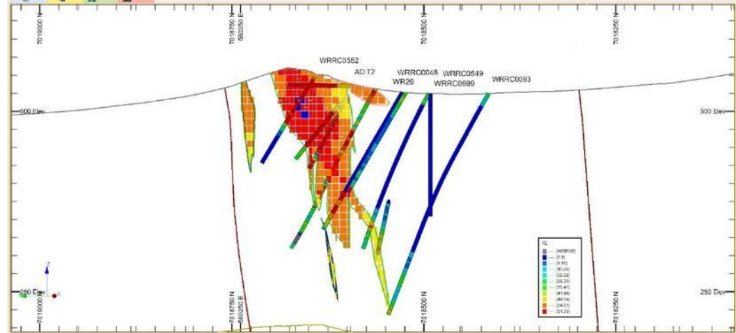
Figure 4. Madoonga section view west facing (E56500)
