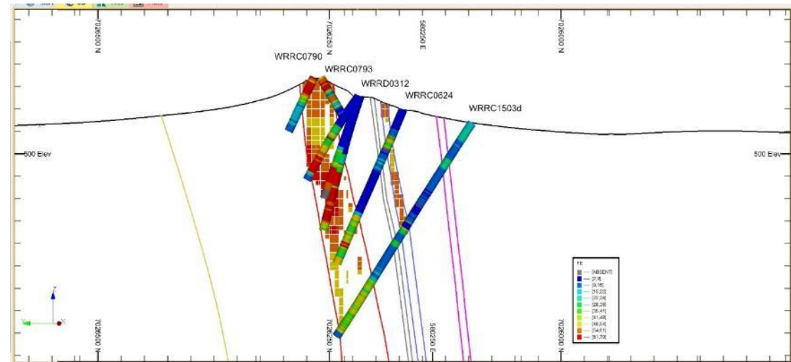
Figure 3. Beebyn North section view west facing (E68500)
