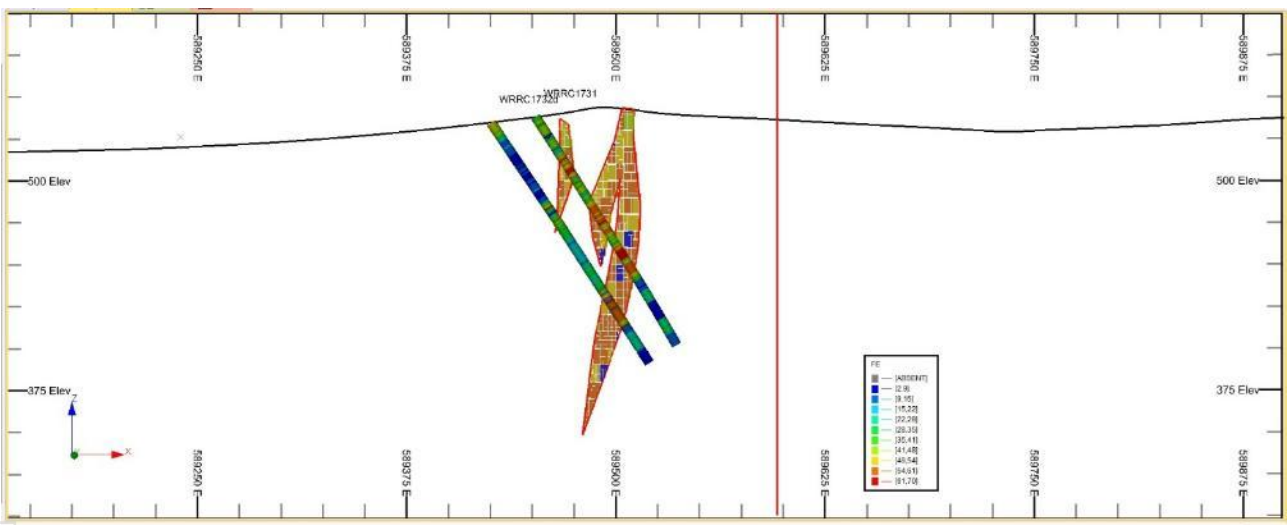
W39/39 section view north facing (N7037750)
