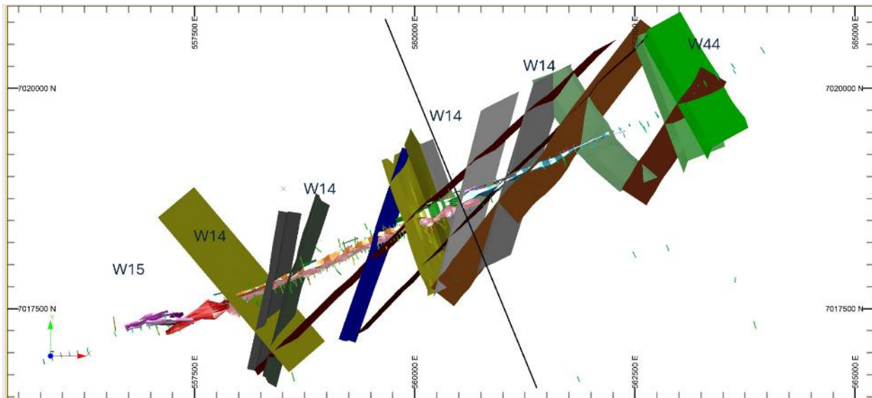
Figure 5. Madoonga deposit structural model (plan view)
