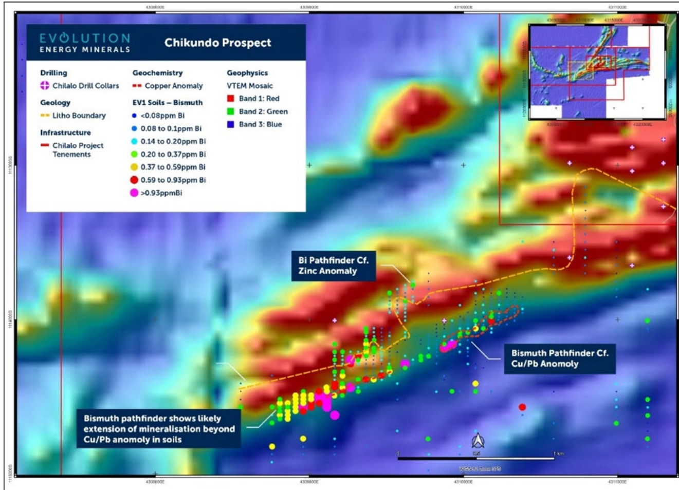
Bismuth Pathfinder chemistry indicating the possible extension of the anomaly to the southwest
