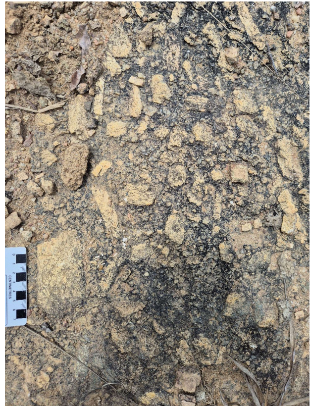
Figure 6: Feldspar phenocrysts in porphyry granite at SAJ-RO-33 sample point
