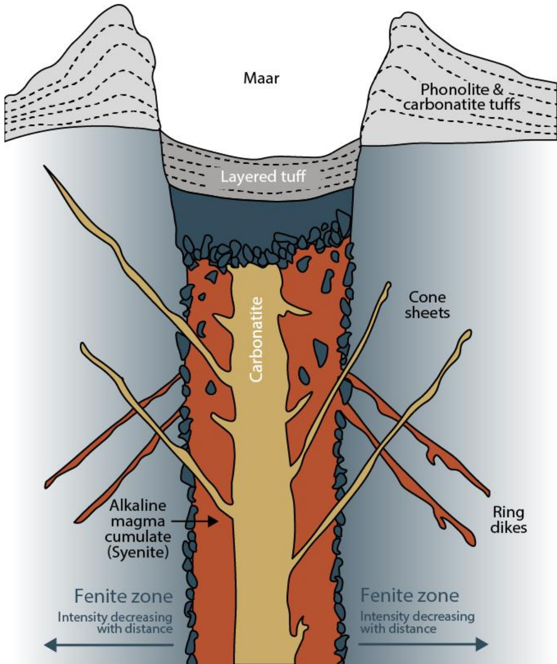
Figure 1 Geological cross section showing carbonatite intrusion, cone sheets, ring dykes and breccia layers. (Credit: graphic adapted from a model for Carbonatite deposits: https://geologyscience.com/geology-branches/magmatic-deposits/ )
