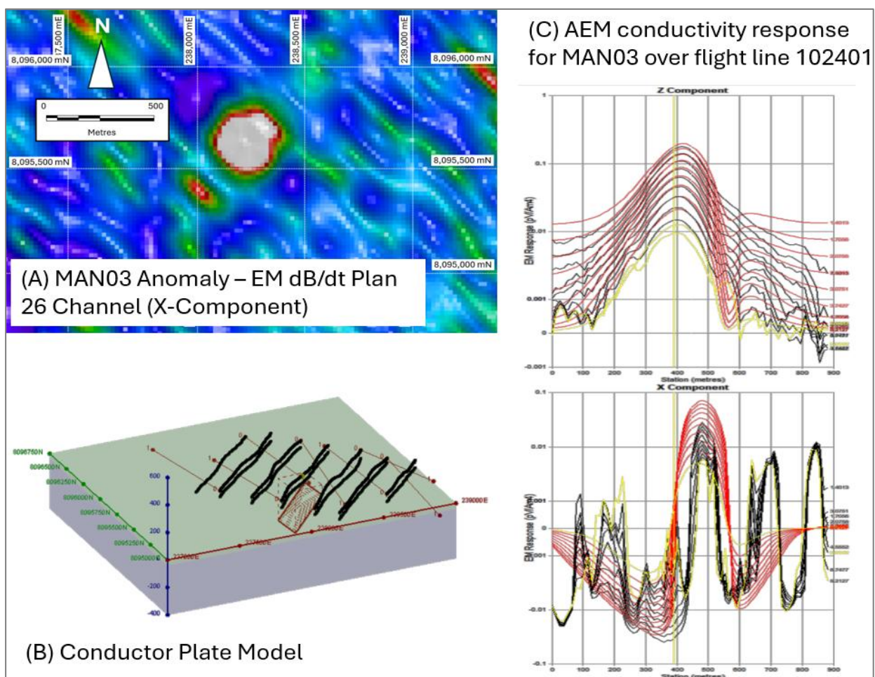
Figure 2 - Maniopotia MAN03 Anomaly, Z- and X-Component response and resultant plate model.
