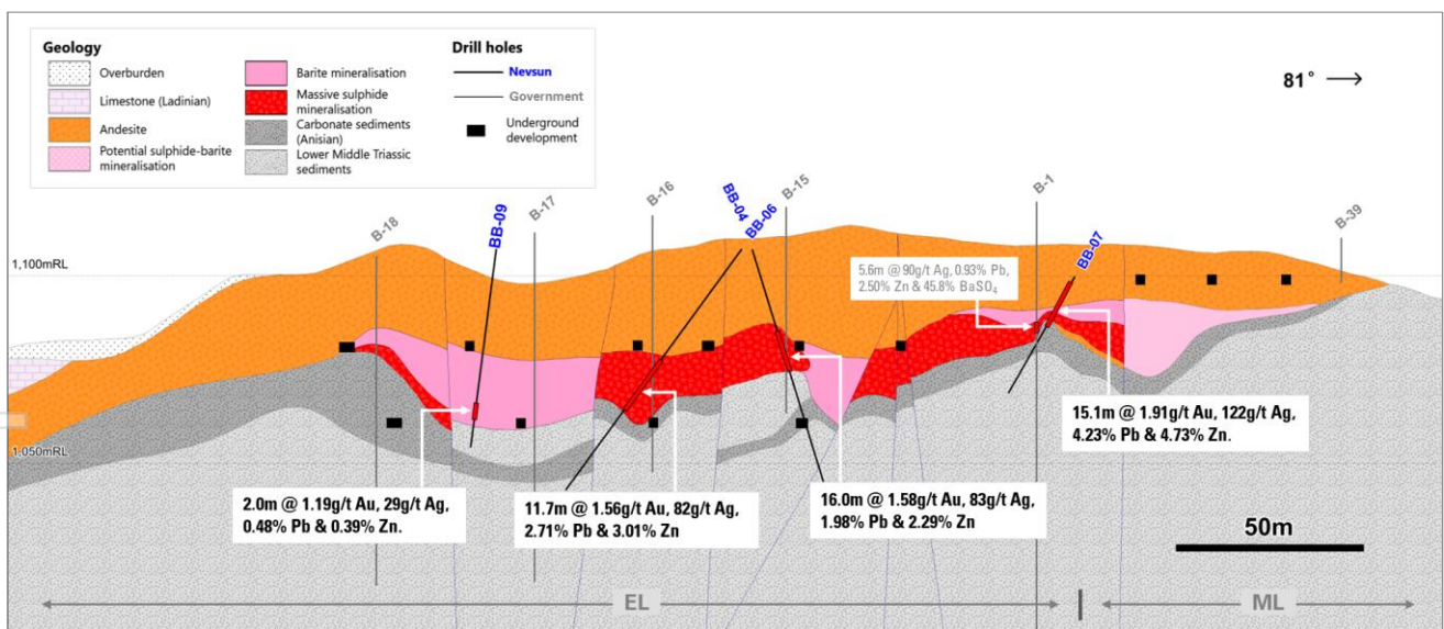
Figure 5: Schematic cross section of Bobija mine area (view to north / 351 deg.) – showing location of historic drilling (after Reservoir Minerals (24 Nov. 2014), Nevsun Resources (Oct. 2016) and Government drill logs).
