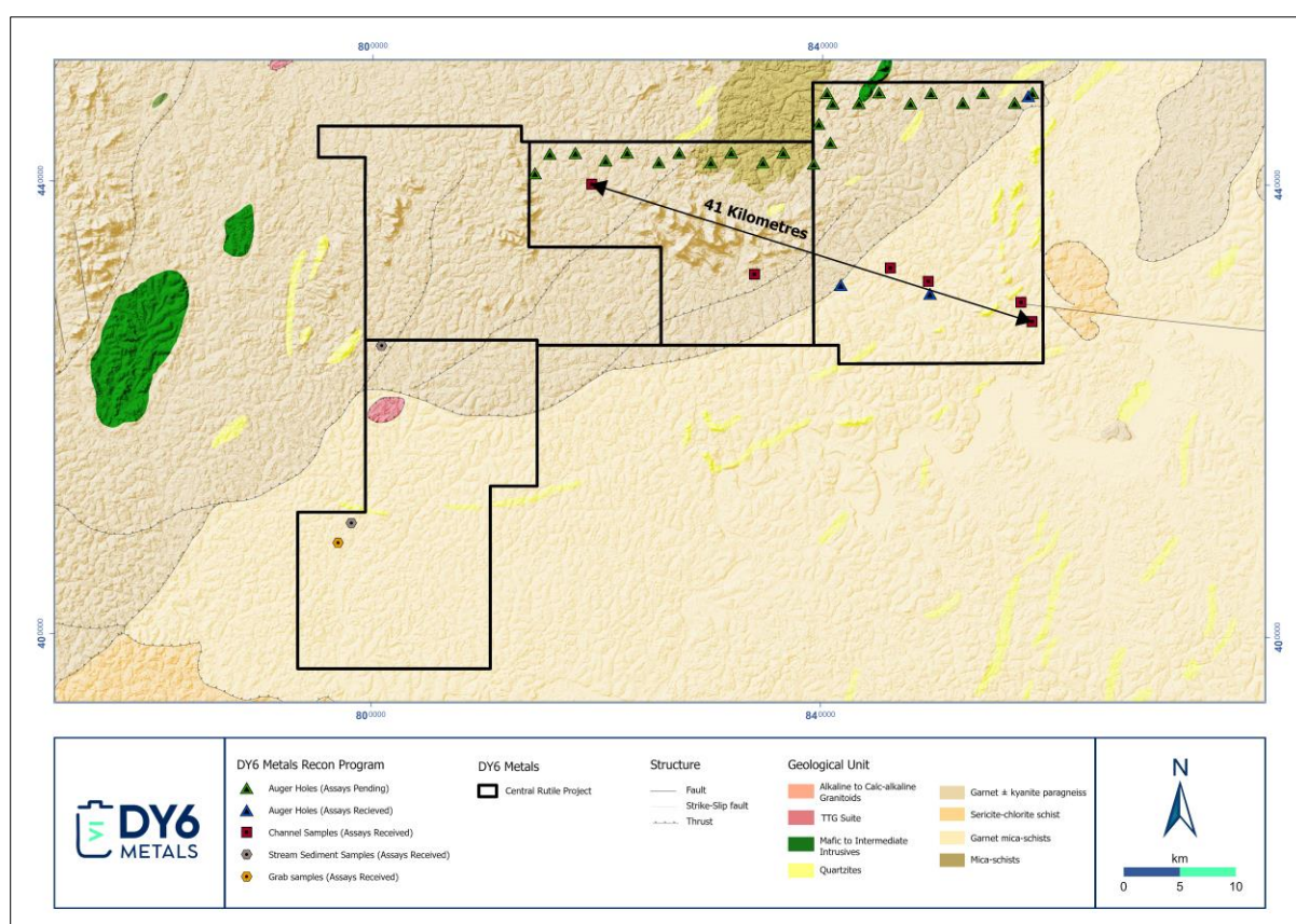
Figure 1: Zoomed in geological map of the Nsimbo and Alamba licences showing the recently completed reconnaissance sampling campaign.
