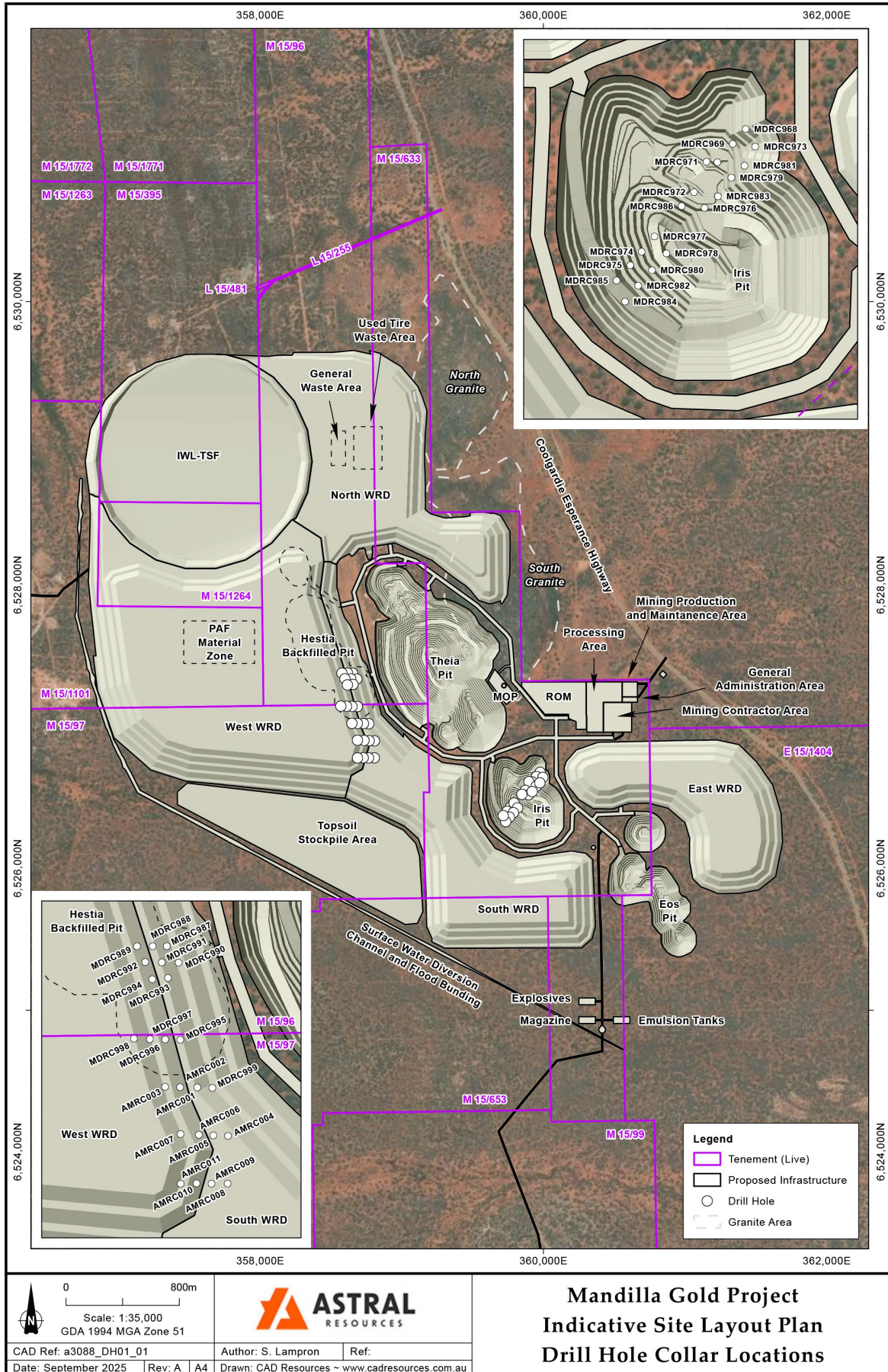
Figure 5 – Mandilla Gold Project infrastructure layout relative to Hestia sterilization drilling
