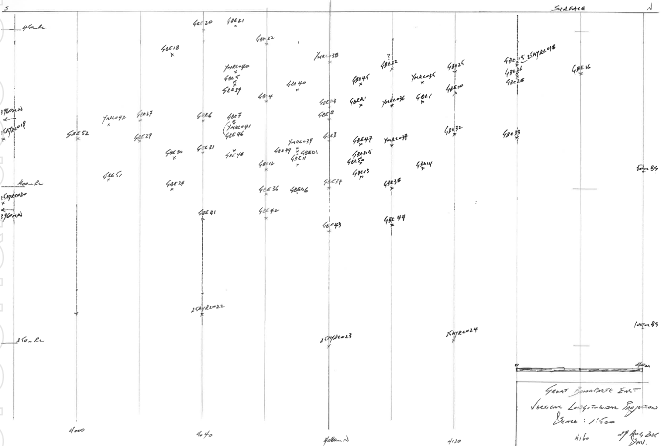
Figure 6: Schematic Vertical Longitudinal Projection (GBE local grid) with recent assay results and historical drilling.
