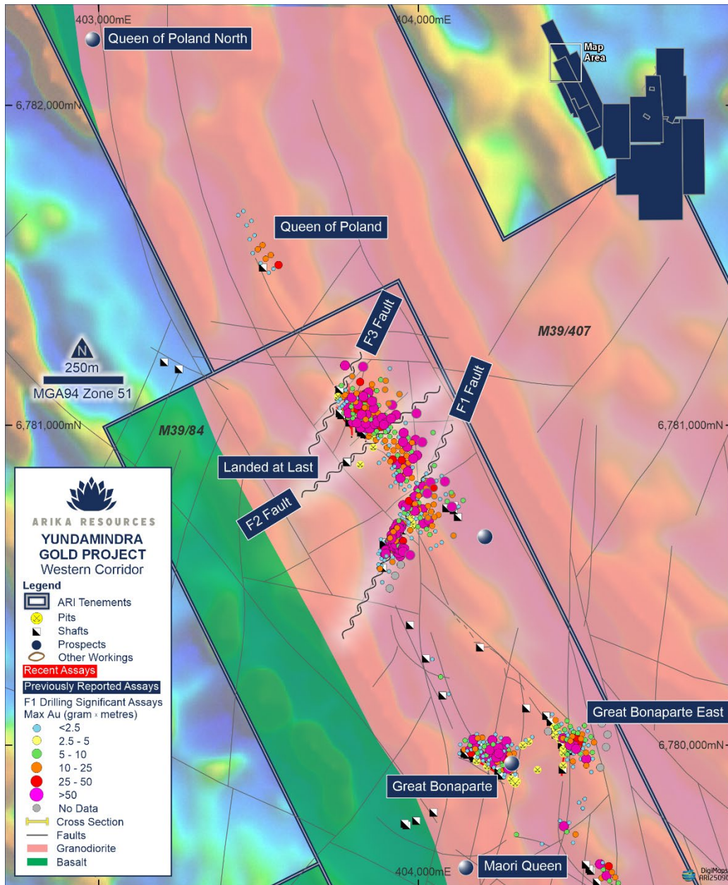
Figure 2: Zoom in of the northern section of 'The Yellow Brick Road', Western Corridor. Prospect Location plan showing recent drilling and proposed holes over simplified geology and TMI.
