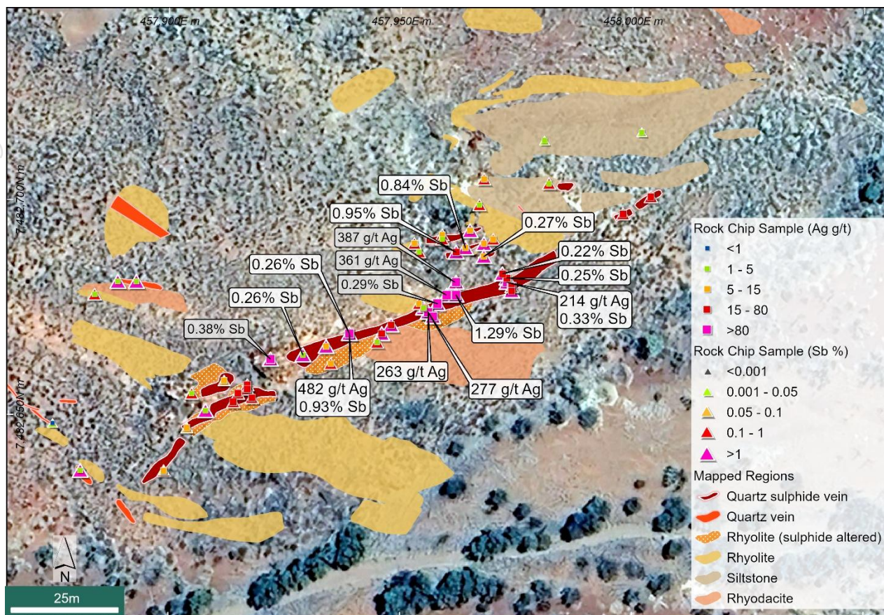
Figure 4 Geological mapping and significant Sb and Ag rock chip results at the SE Wyloo prospect (results in grey previously reported – Refer to Novo’s ASX announcement dated 11 September 2024 – Evaluation of Pilbara Antimony-Gold potential generates positive results)
