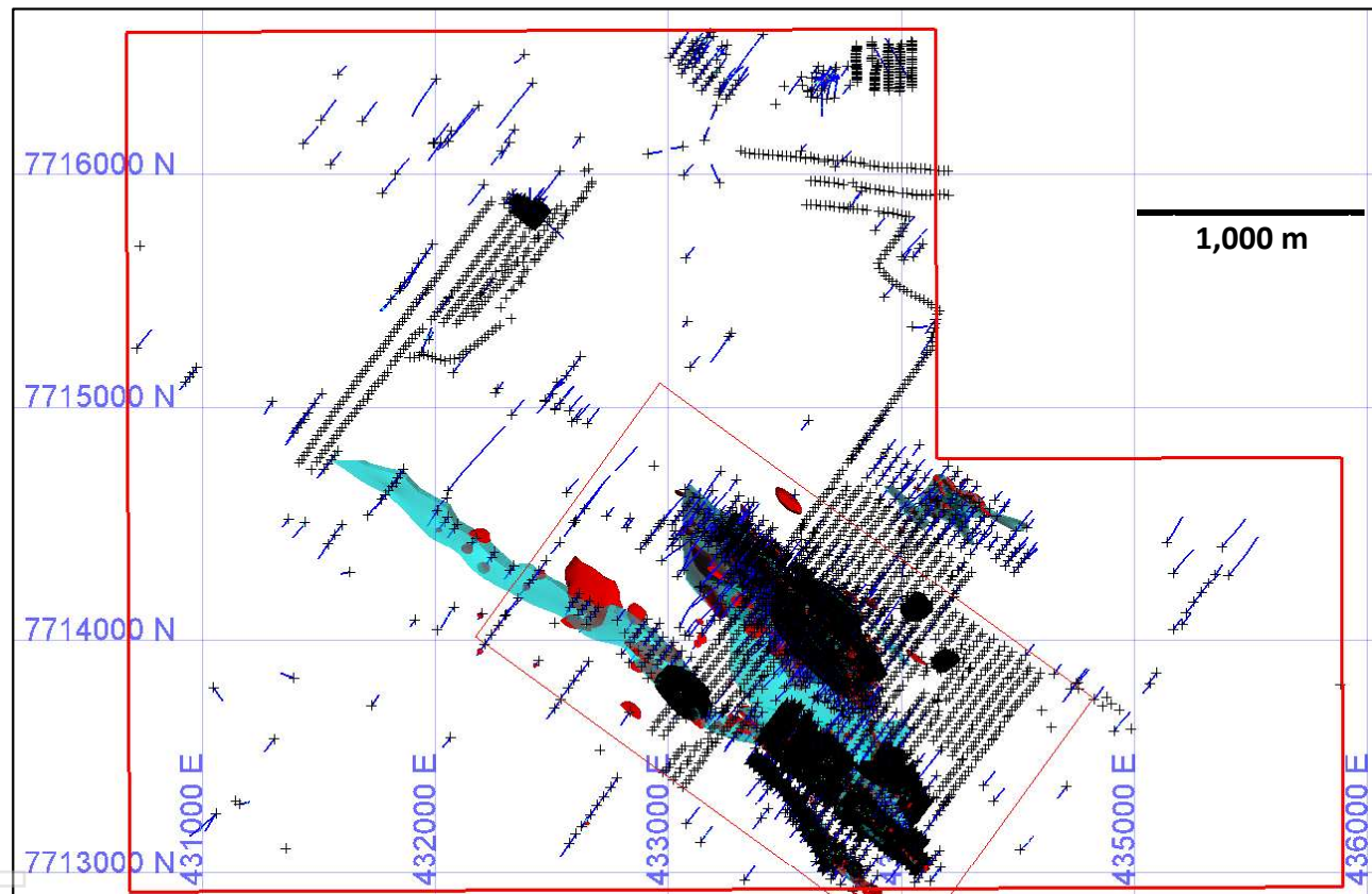
Figure 10-7. Plan view of drilling on the Rocklands ML.
