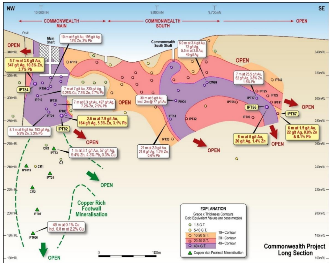
Figure 2: Commonwealth Long Section showing drill hole pierce points, and grade times thickness values for mineralisation between Main Shaft and Commonwealth South.
