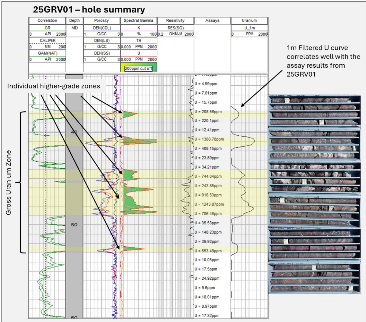
Figure 4: 25GRV01 down-hole spectral gamma log, chemical assays and core photos
