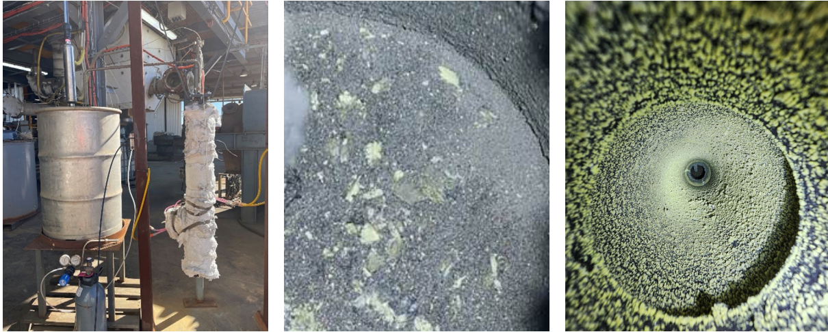
Figure 4 - (L-R) Vertical kiln prototypes, pyrrhotite product after pyrite conversion and sulphur collection in condenser.
