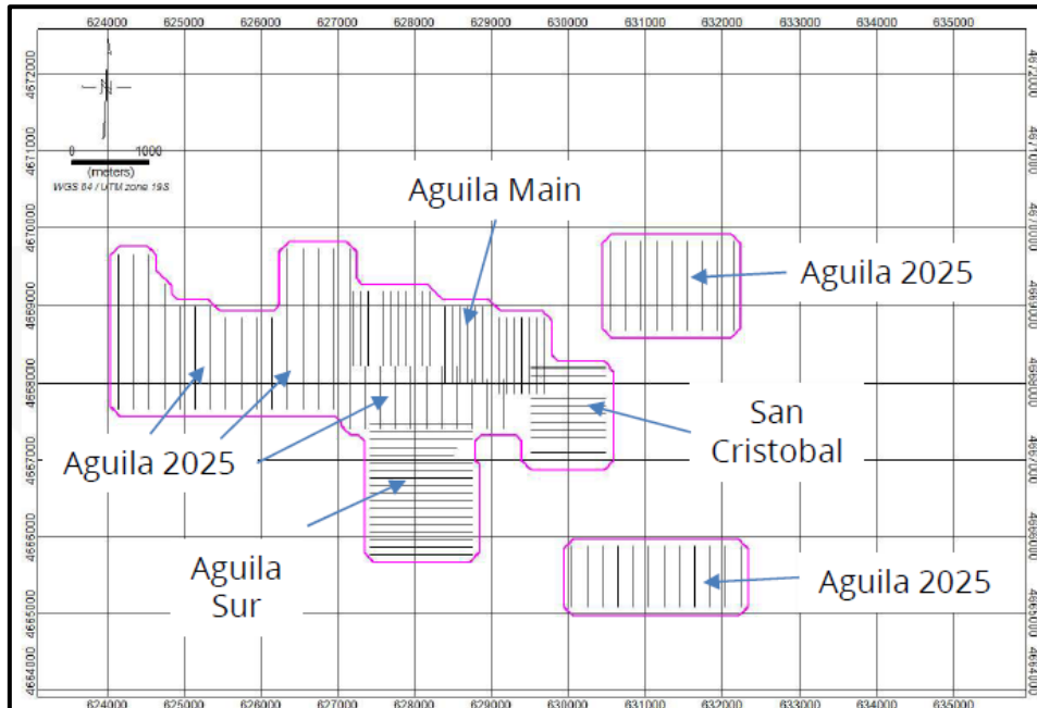
Figure 9: El Aguilá project induced polarization survey grids, line orientations and date of the survey.
