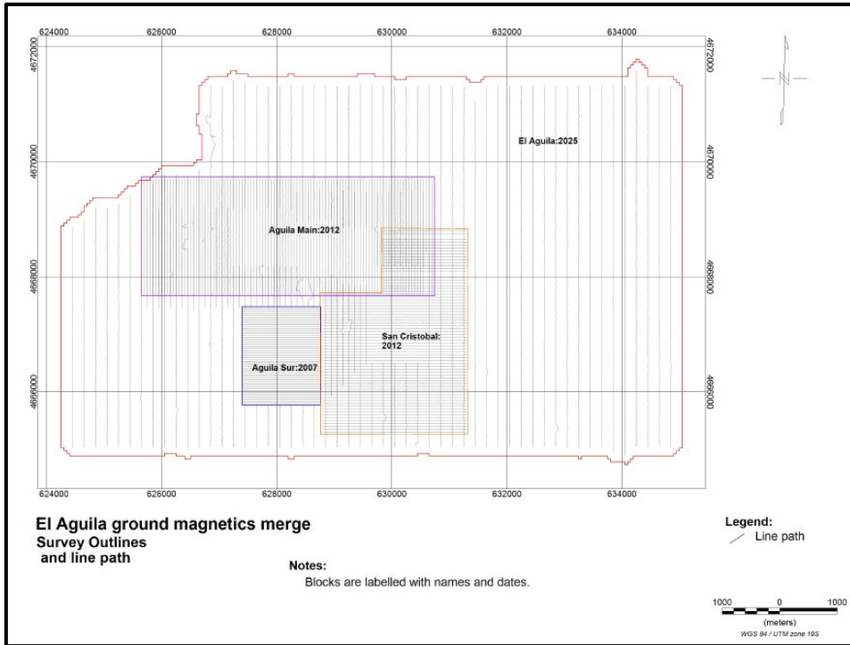
Figure 8: El Aguilá project magnetic survey grids, line orientations, and date of the survey.
