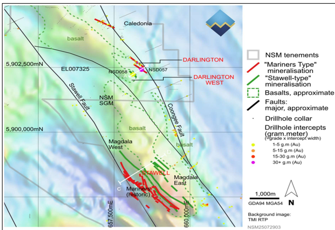
Figure 1 Geology, mineralised trends and magnetics data showing the interpreted relationship between the Stawell Mine (SGM) and Darlington and Caledonia prospects (NSM).
