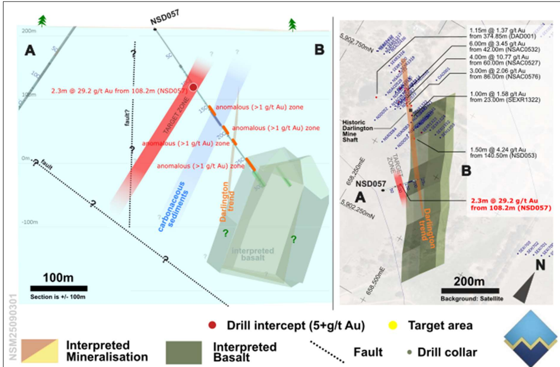
Figure 2 NSD057 - plan and section (+/- 100m). Target zone around NSD057. The brecciated quartz-sulphide-gold intercept is interpreted as similar mineralogy and structure to the descriptions of the Mariners Lodes, 6km to the south at Stawell.
