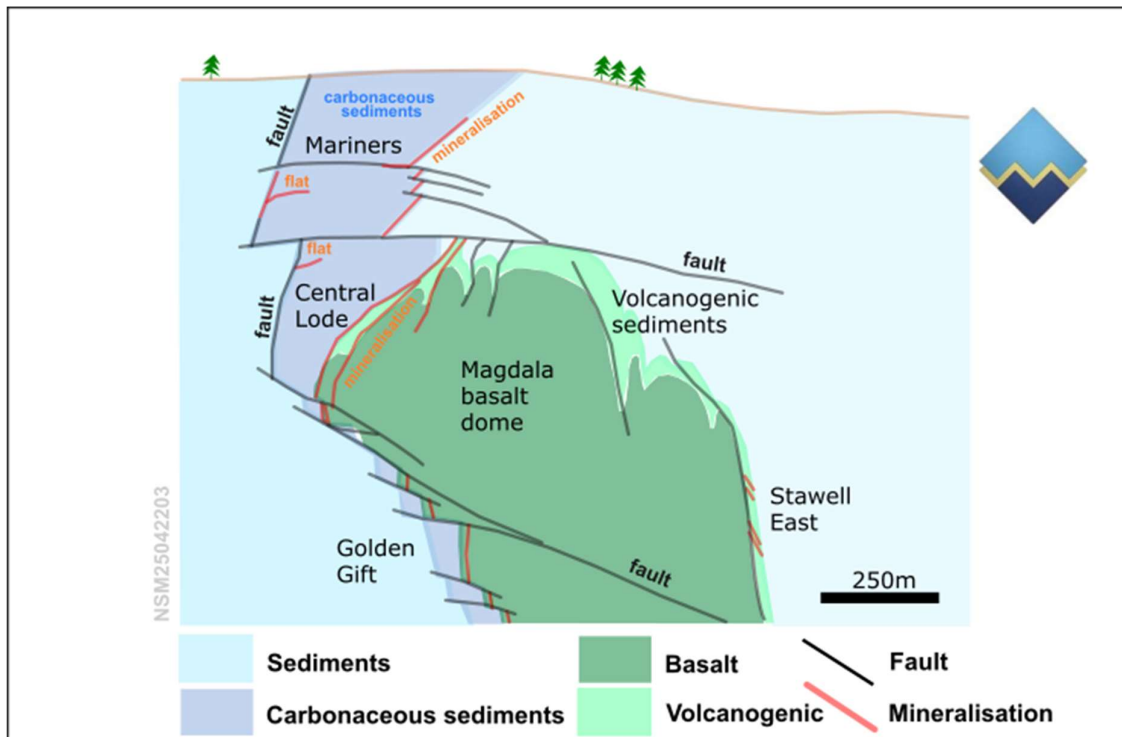
Figure 3 Simplified cross section through the Mariners Lodes (aka. hanging wall lodes). The figure demonstrates the relationship between the Mariners-type mineralisation, geology, faulting and the deeper basalt-associated (Stawell-type) mineralisation (aka Central Lode and Golden Gift). The mineralisation in the Mariners Lode is characterised by brecciated quartz and abundant visible gold.
