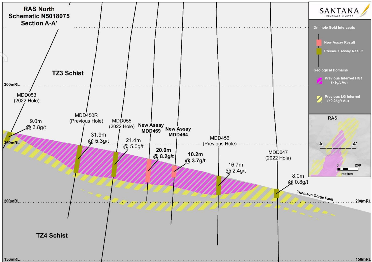
Figure 2. Schematic cross section at 5018075N showing new drilling.
