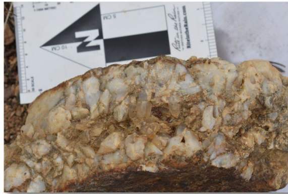
High-level quartz veining texture. Note crystal growth.
