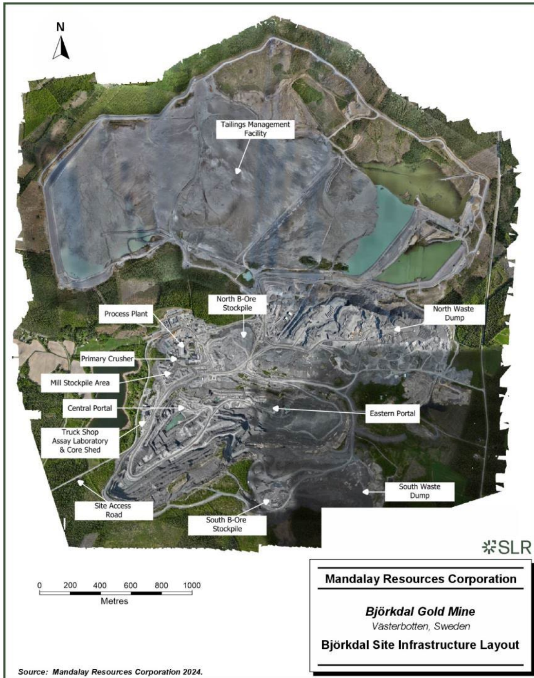
Figure 18-1: Björkdal Site Infrastructure Layout
