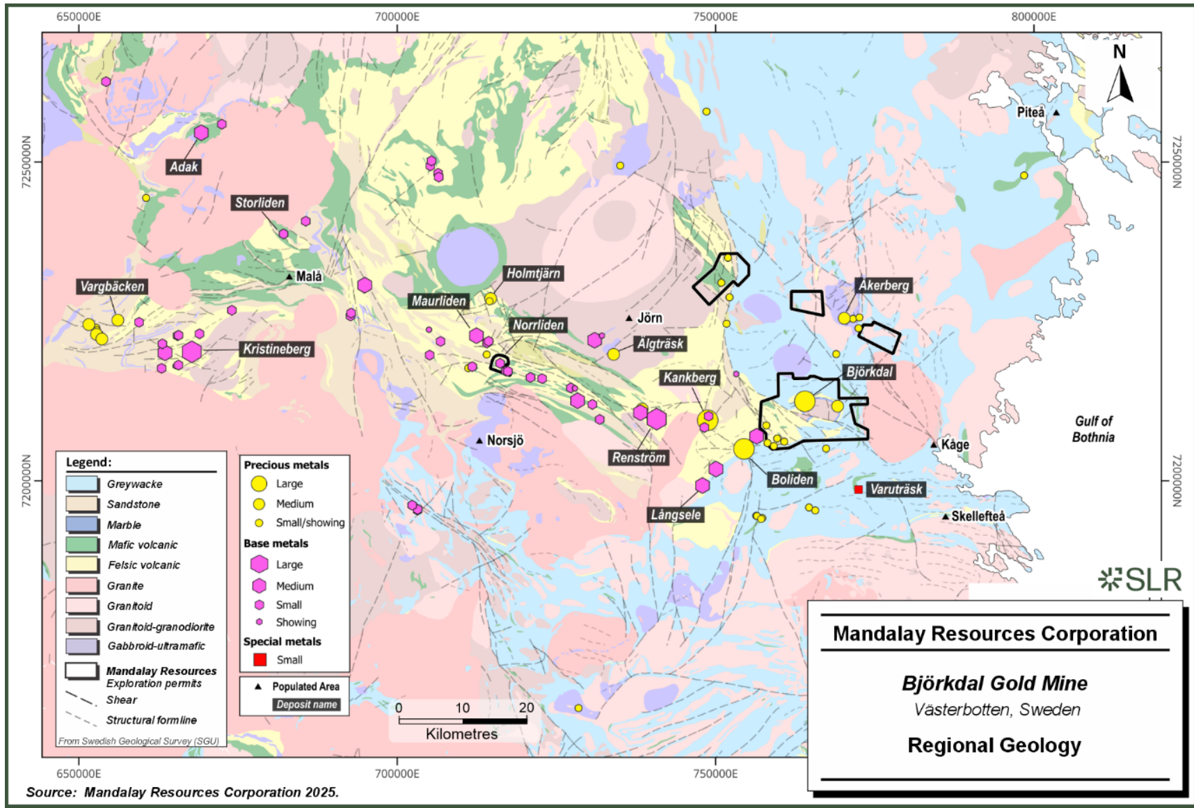
Figure 7-1: Regional Geology
