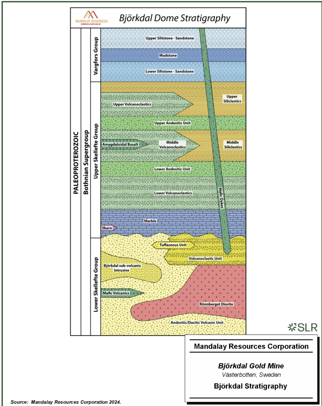
Figure 7-3: Björkdal Stratigraphy
