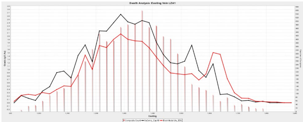
Figure 14-17: Swath Plot by Easting, Vein LZA1 (Aurora)
