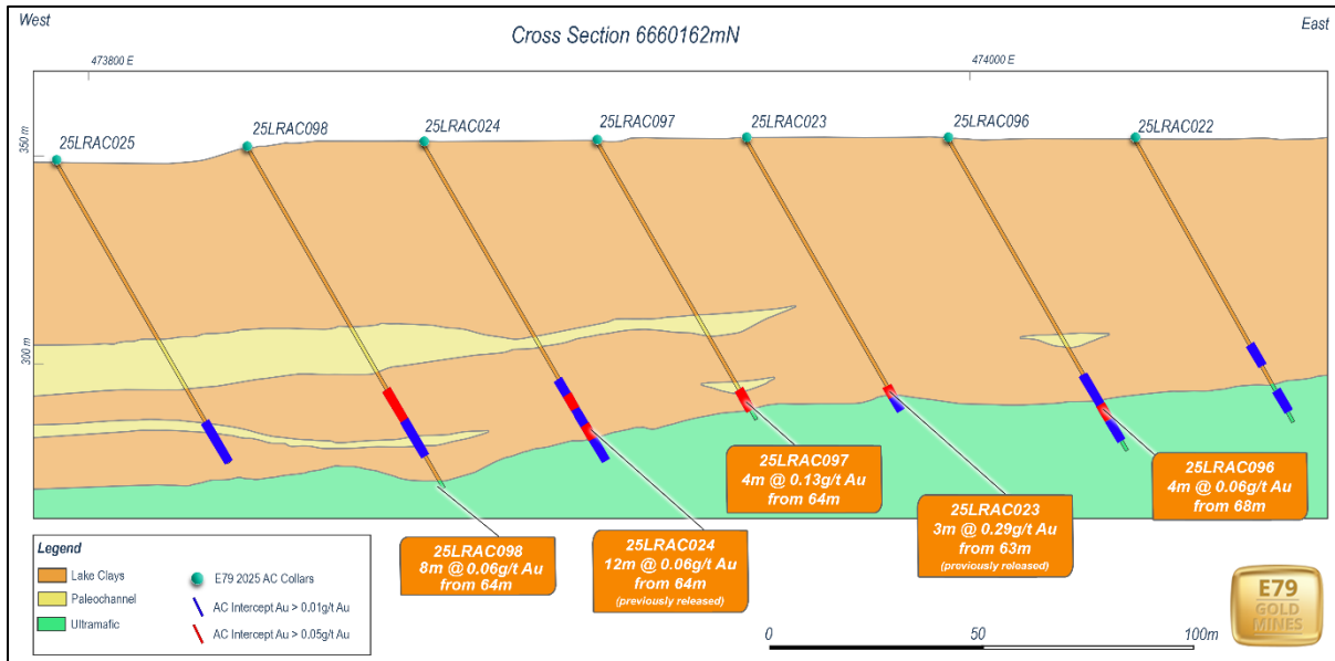
Figure 5. Cross-section of drill line 6660162mN.
