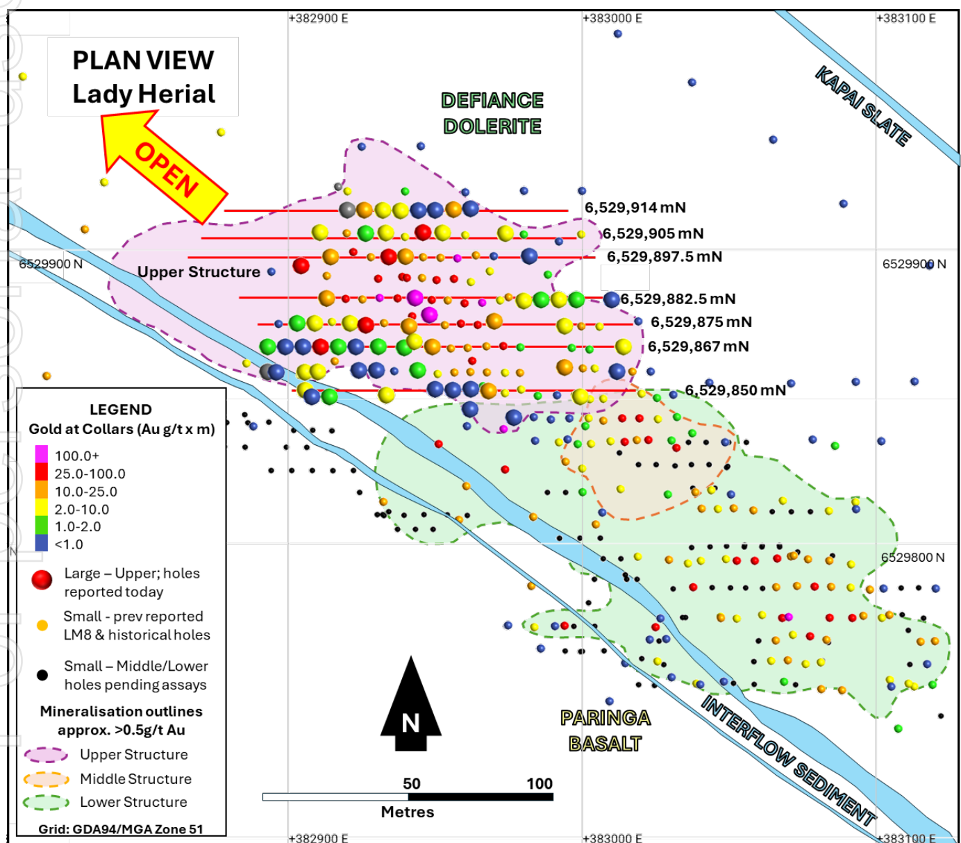
Figure 1: Plan View of the Upper Structure at Lady Herial showing recent grade control spaced results and the section numbers and locations of Figures 2 through 8.
