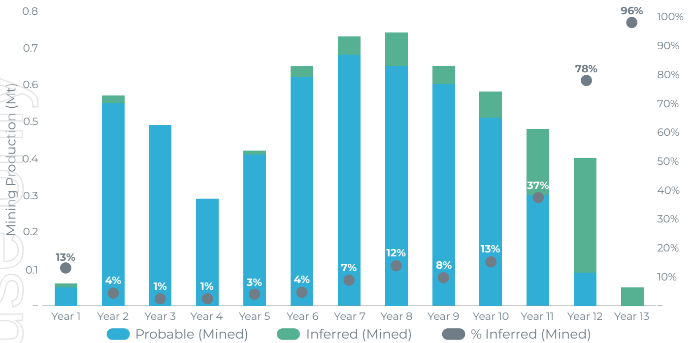
Figure 11 Mined Production Plan by Categories
