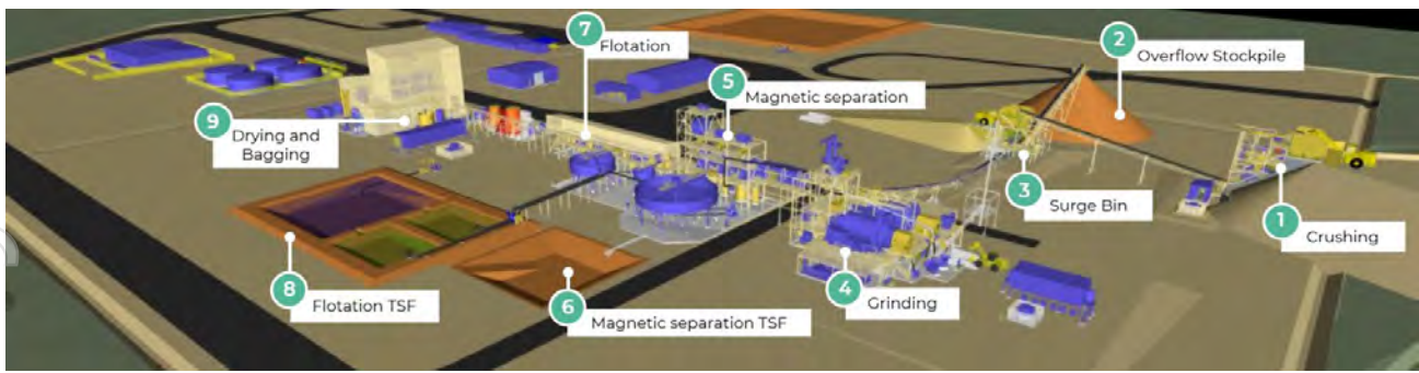
Figure 6 Plant layout
