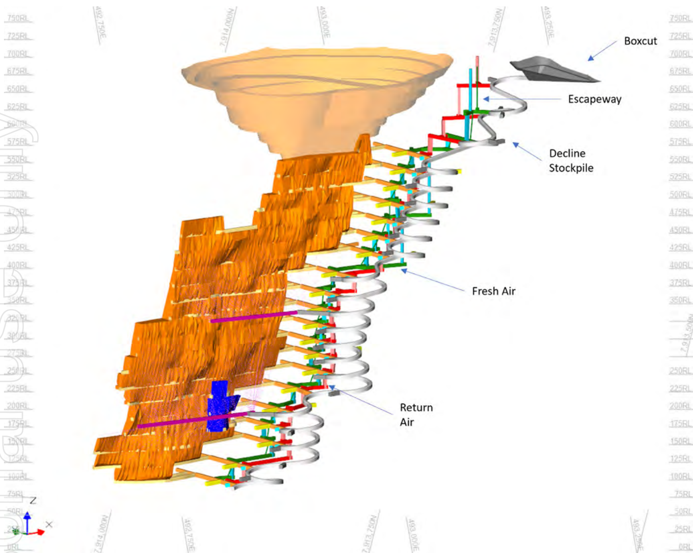
Figure 15 Proposed Wolverine underground mine layout
