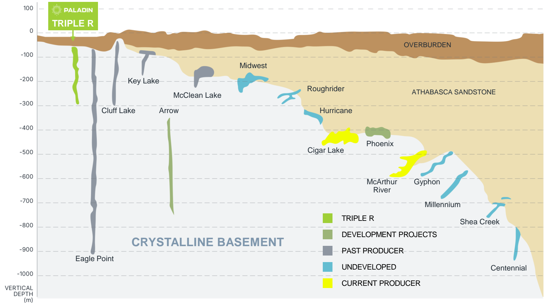
Athabasca Basin regional deposits
