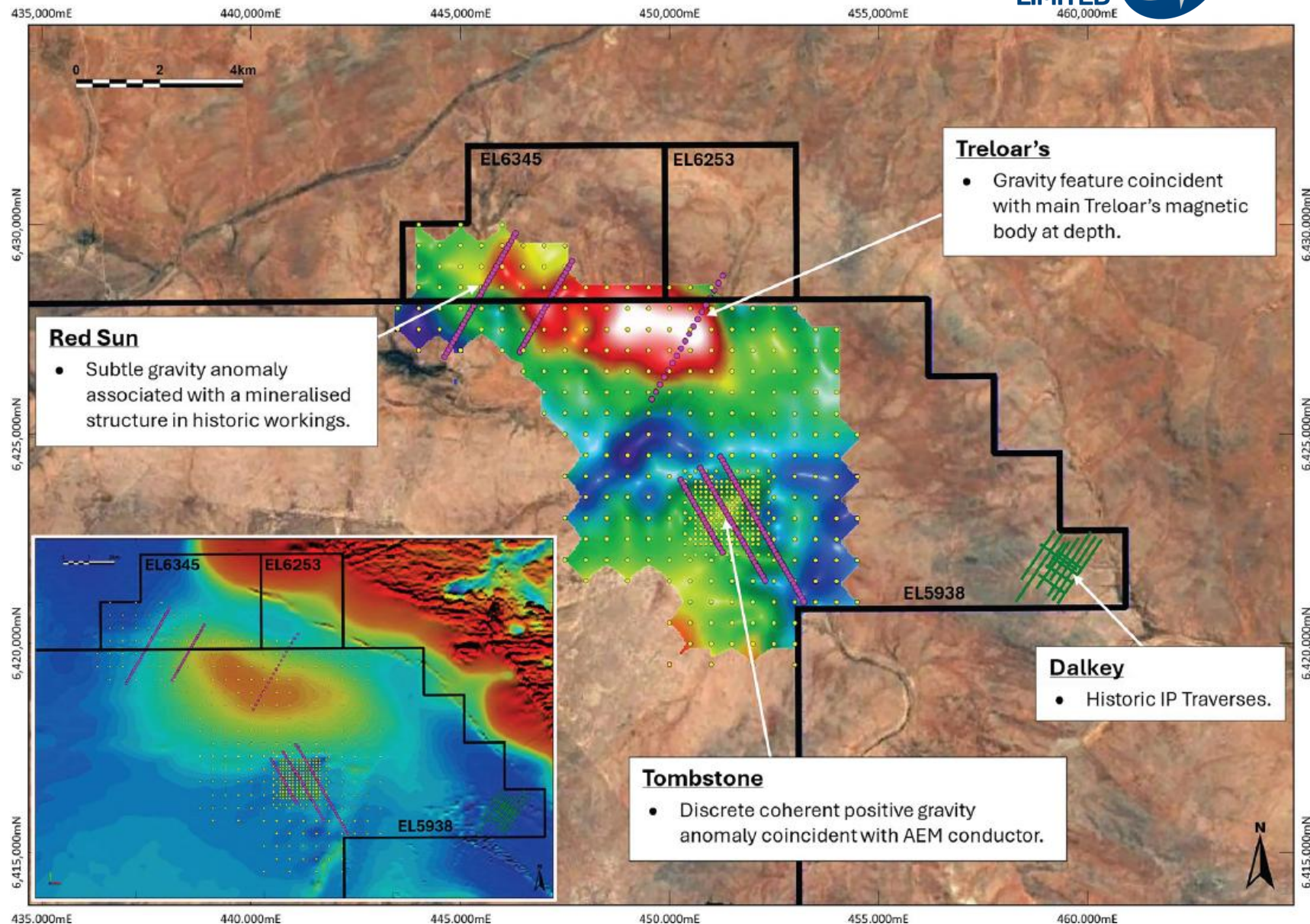
Band pass filtered gravity data, with new IP traverses shown in pink.
