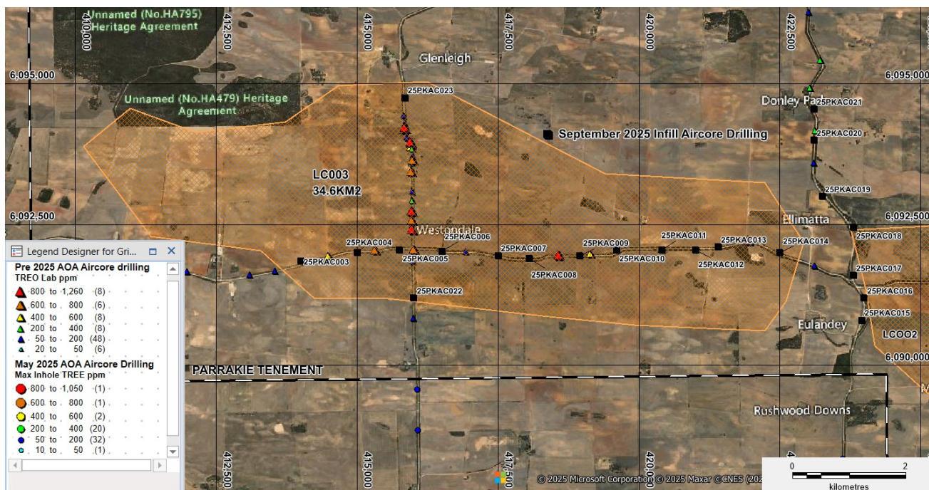
Figure 3: Parrakie Area LC003(Jabuk) – Showing historic drilling and drilling for September 2025
