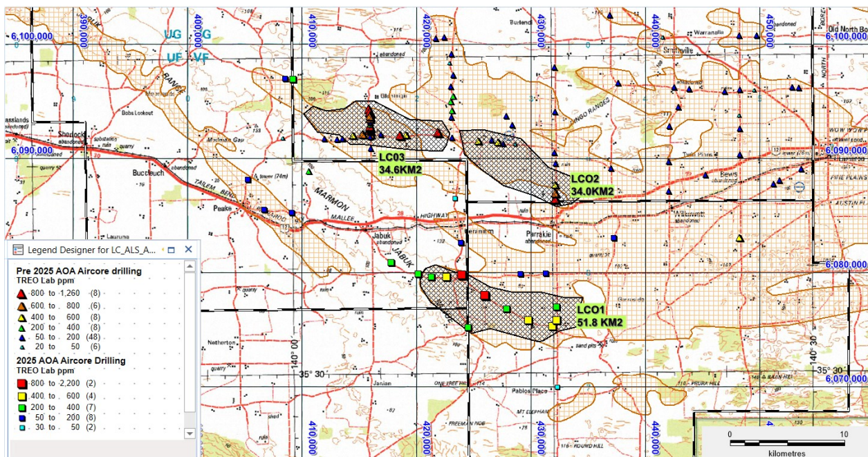
Figure 2: Maximum ppm TREO in the May 2025 and 2024 Aircore drilling programs that targeted the potentially REEs mineralised Loxton Parilla Sands (brown)
