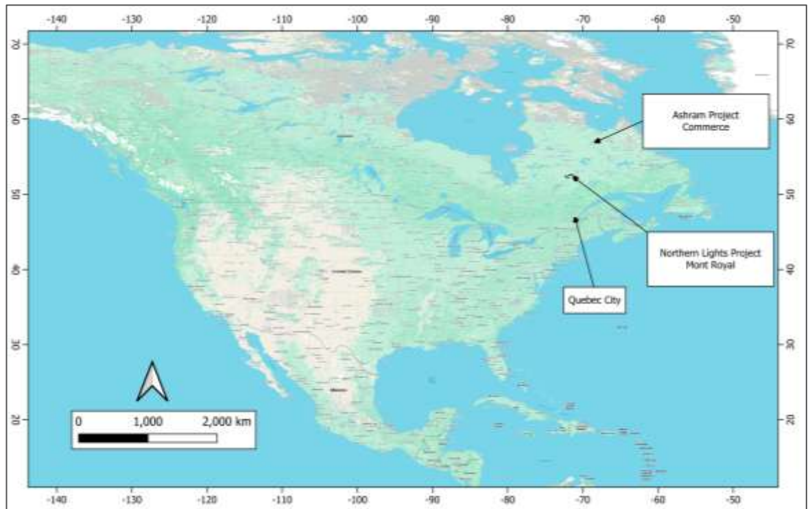
Figure 1.1: Location of the subject mineral assets
