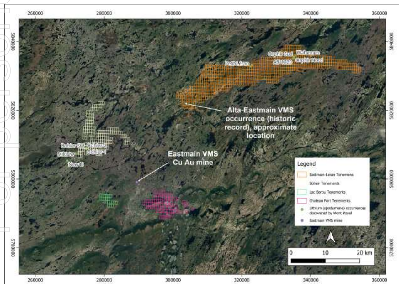
Figure 3.3: Mont Royal lithium (spodumene) mapped occurrences
