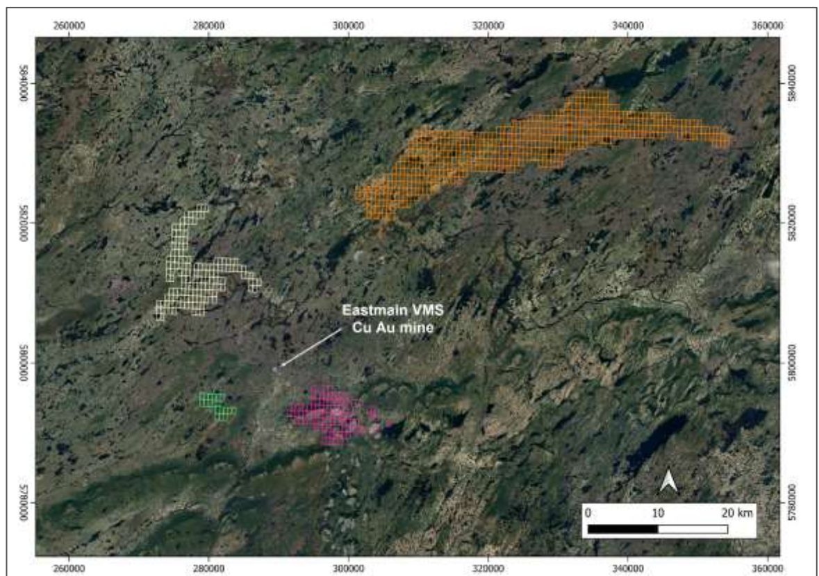
Figure 3.2: Location of Eastmain volcanogenic massive sulfide mine
