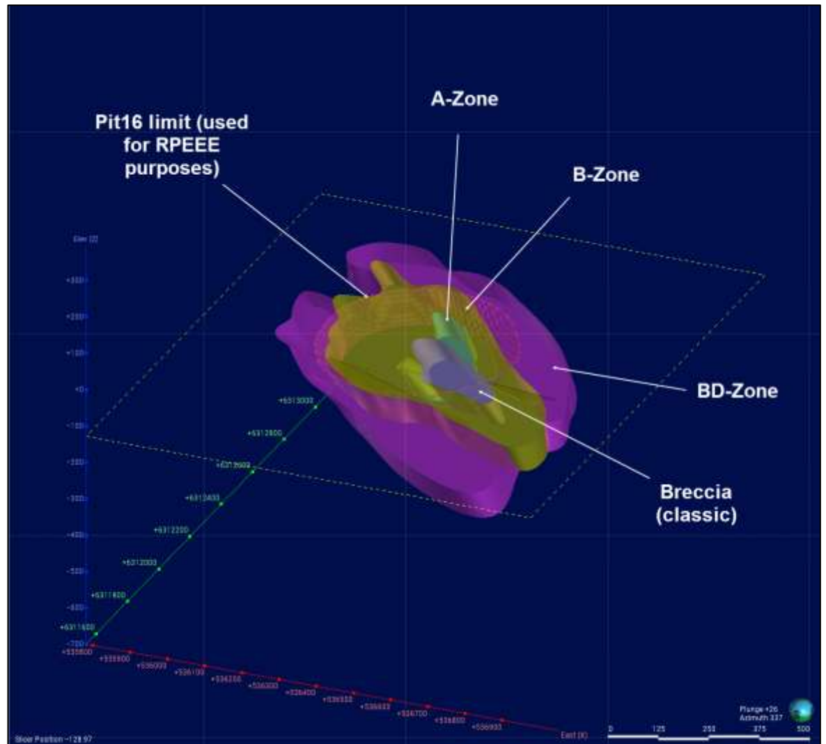
Figure 4.4: Mineralised domains at Ashram
