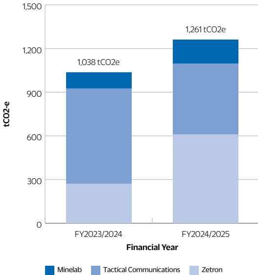
Figure 4: Scope 2 emissions by reporting group
