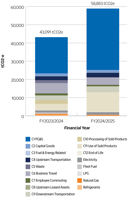
Figure 2: Year on Year emissions breakdown by Category
