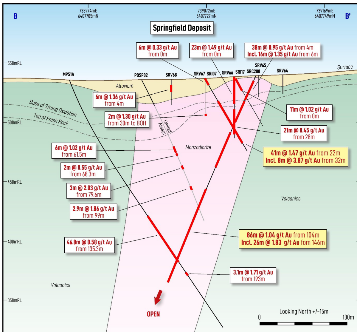
Figure 3. Cross section B-B' illustrating mineralisation at the Springfield Gold Deposit. Mineralisation remains open in all directions. (See Figure 1 for location of cross section).
