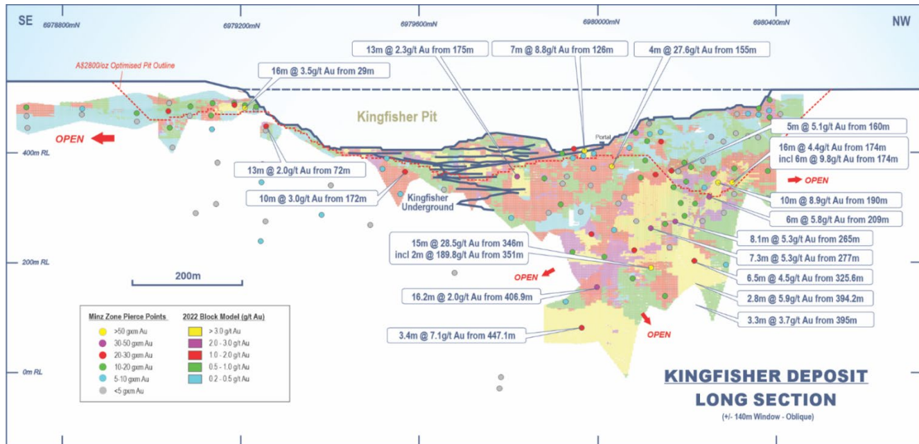
Figure 14: Kingfisher long section showing gold intercept gram x metre pierce points, historic open pit, A$2,800/oz optimised pit shell, and current block model coloured by gold (g/t).
