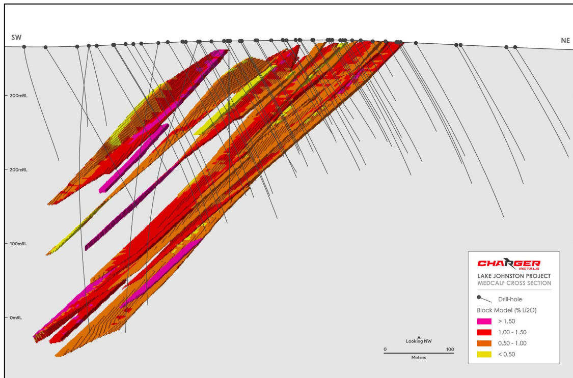
Figure 2. Cross sectional view of the Medcalf Lithium Mineral Resource 8.2Mt @ 1.0% \text{Li}_2\text{O} .
