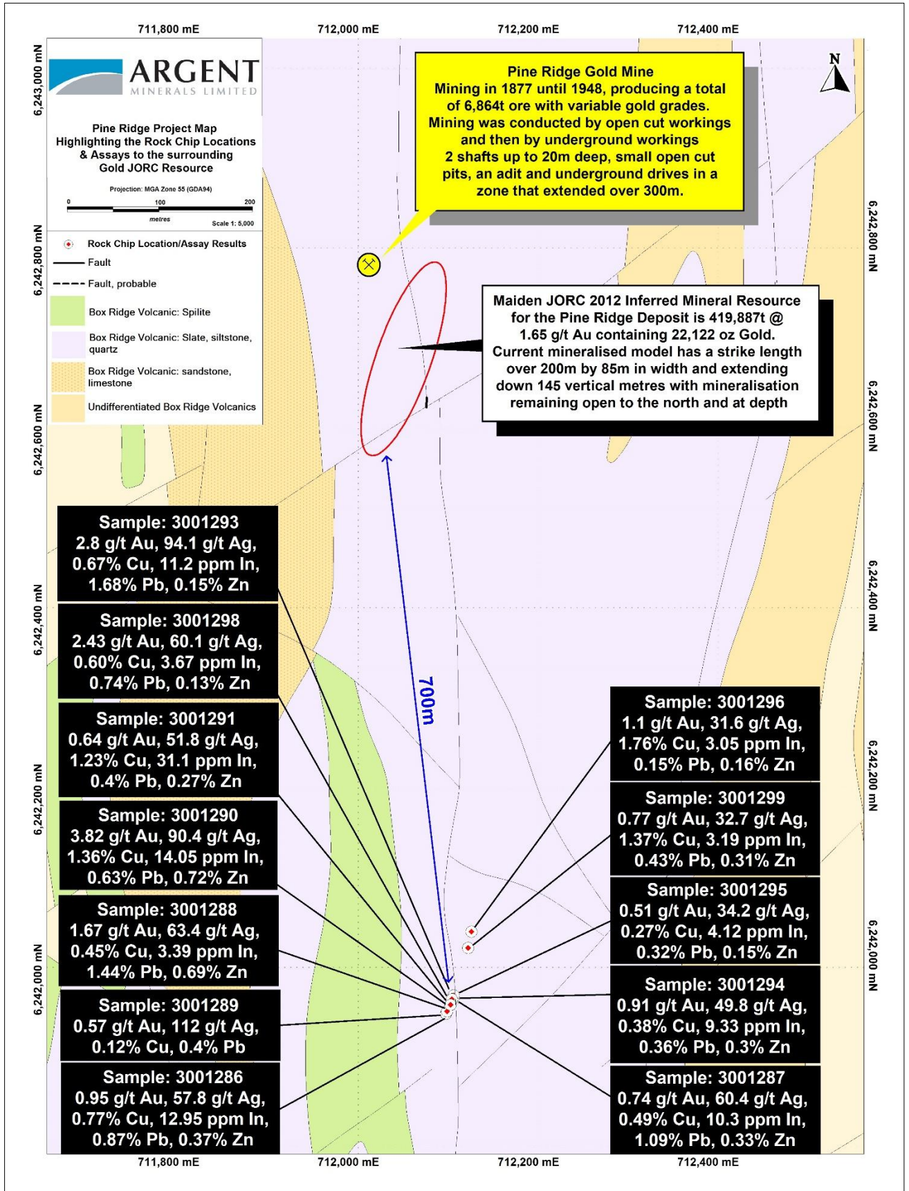
Figure 32 – Pine Ridge/Wood Gully Gossan area highlighting high-grade polymetallic rock chip results – the Wood Gully Gossan is located 700m south of Pine Ridge Gold Deposit
