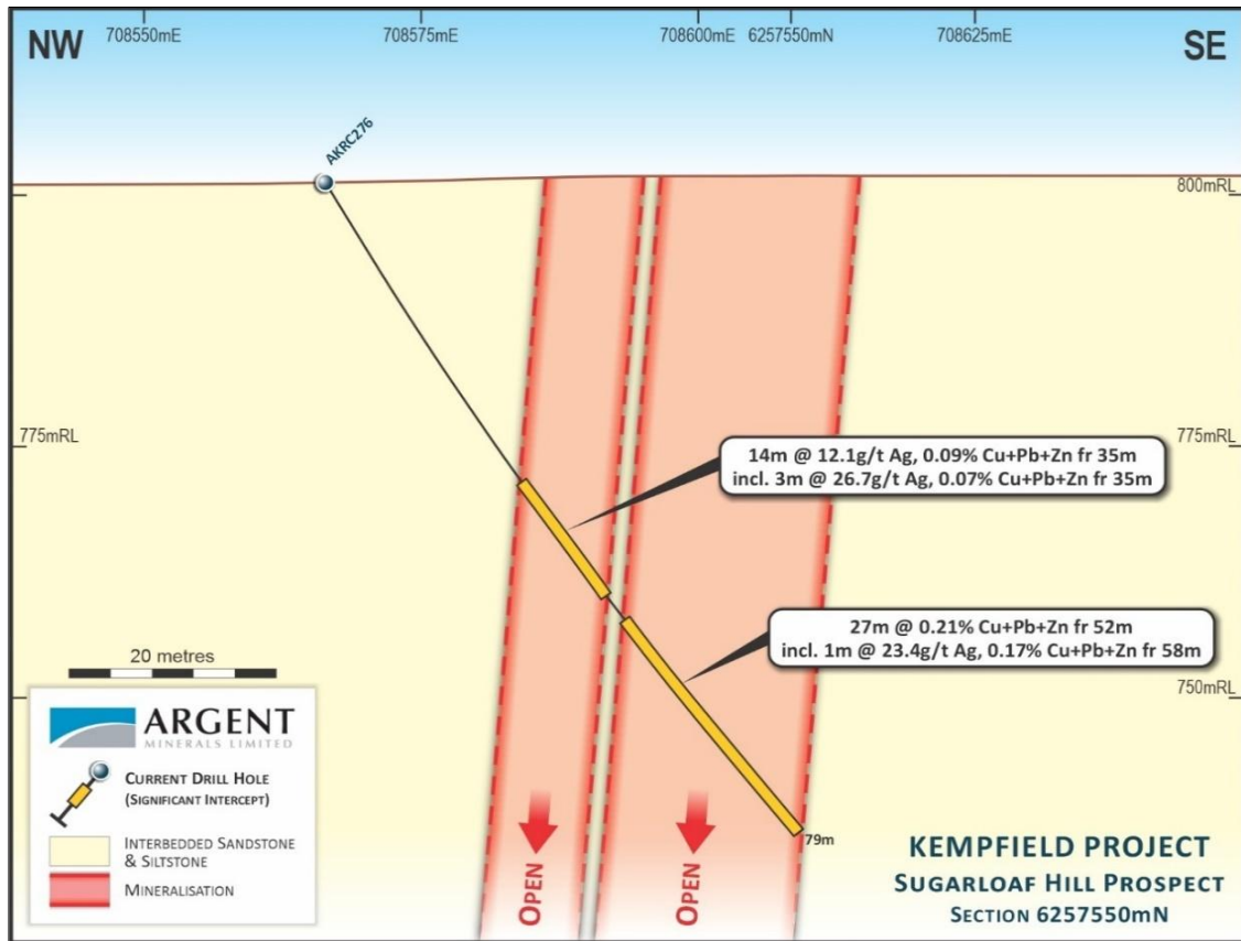
Figure 16 – Sugarloaf Hill Cross Section 625850N highlighting mineralised intervals
