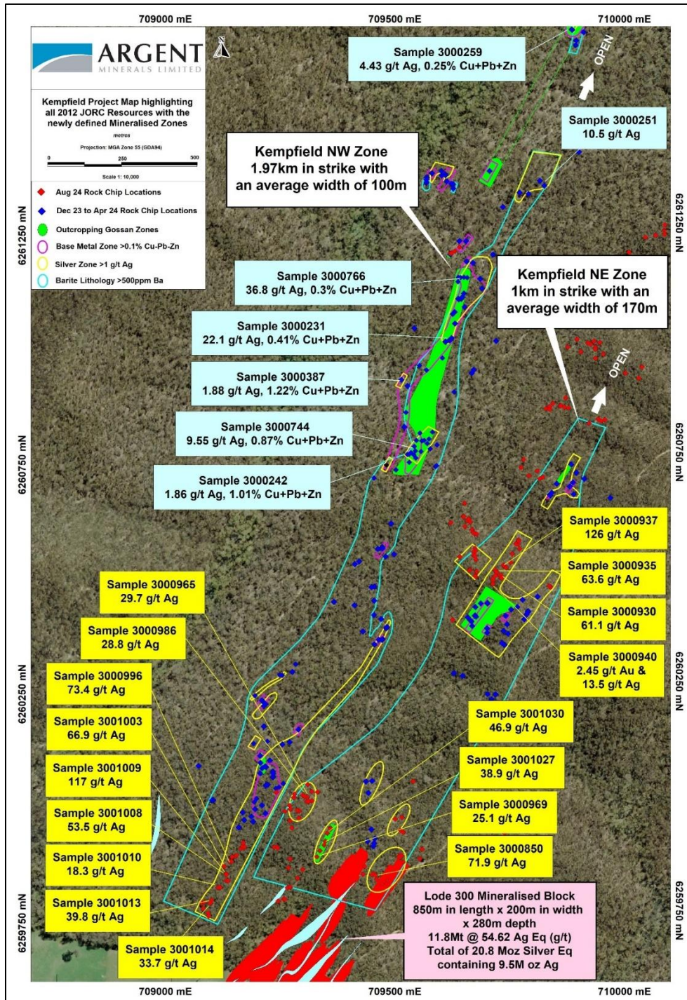
Figure 22 - Kempfield NW and NE Zones highlighting the recent high-grade rock chip results (red colour dots)
