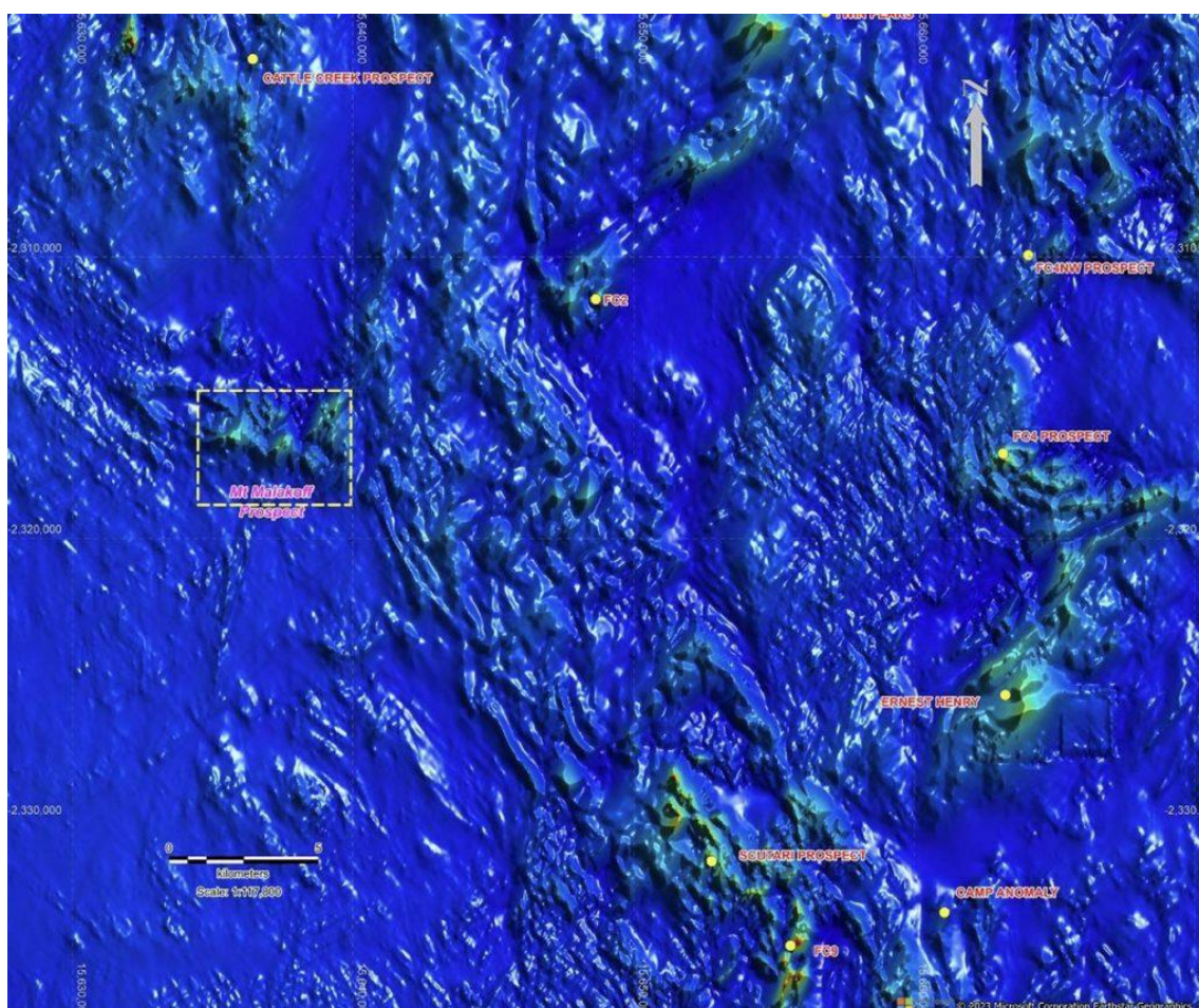
Figure 6: Mt Malakoff Prospect on airborne magnetic map illustrating significant IOCG mineralisations in Ernest Henry area.
