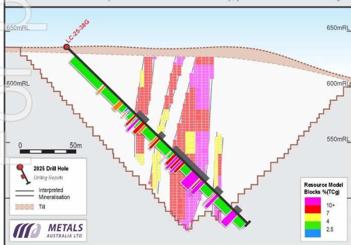
Fig 3: LC-25-38G (Southeastern zone) & Fig 4: LC-25-46 (Connector zone): Figures show downhole log of graphite zones and related mineralisation ((Cu + Pb + Zn + V + Ni Combined basis) & Silver – g/t) and Cross Section of each hole shown beneath the log.
