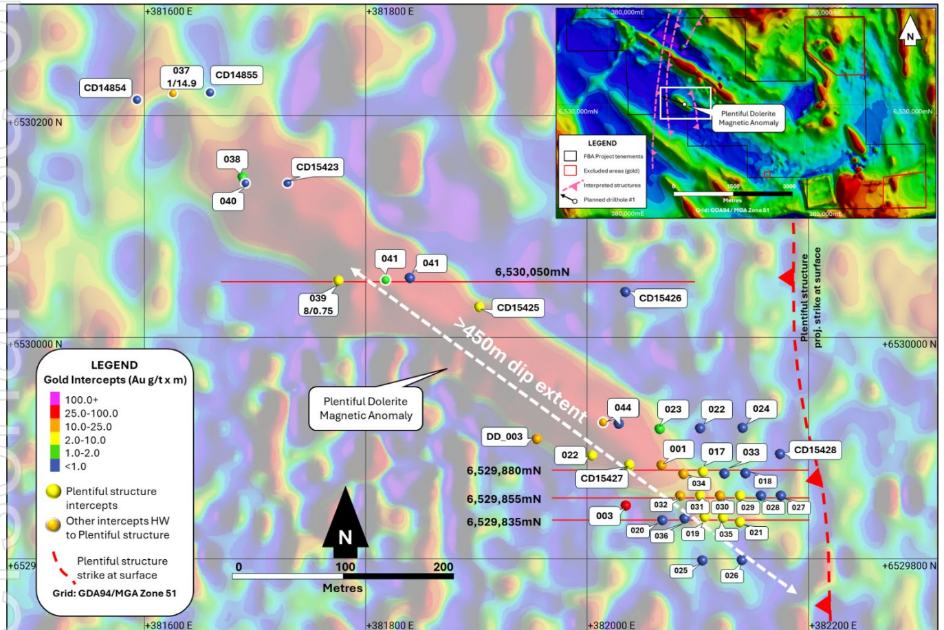
Figure 2: Plan view of the Plentiful dolerite and gold prospect area, showing drill hole IDs and section lines of Figures 4 to 7, over ground magnetic image (reduced to pole – 1 st vertical derivative) with insert displaying location at the project scale and the first planned Plentiful EIS hole.
