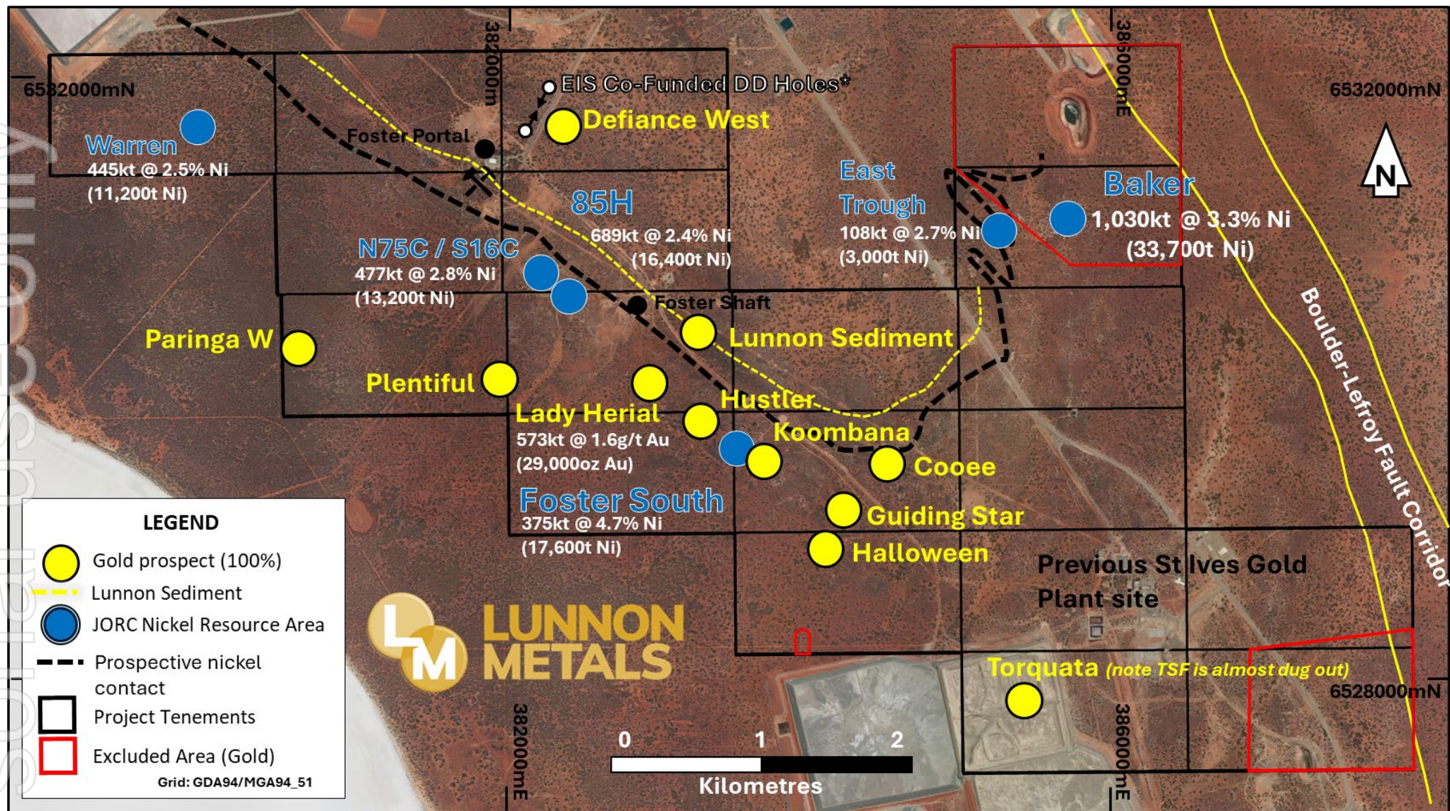
Figure 8: Foster-Baker Project Area showing select high-ranking gold prospects, gold & nickel Mineral Resource 6 positions.
