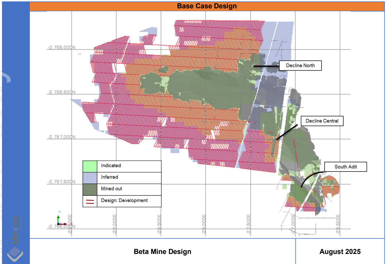
Figure 7: Beta Mine Design
