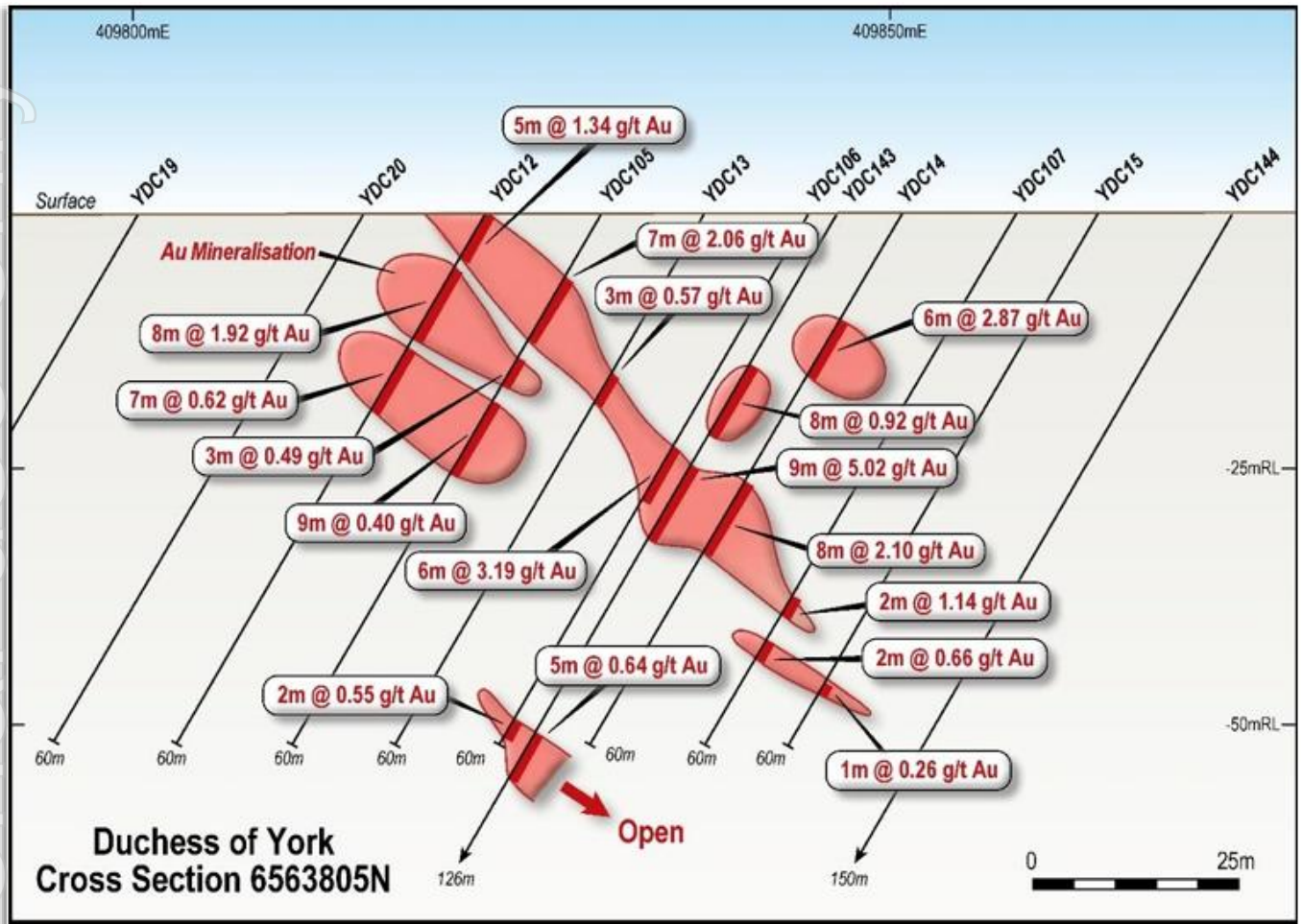
Figure 4: Duchess of York Cross-Section 6563805N
