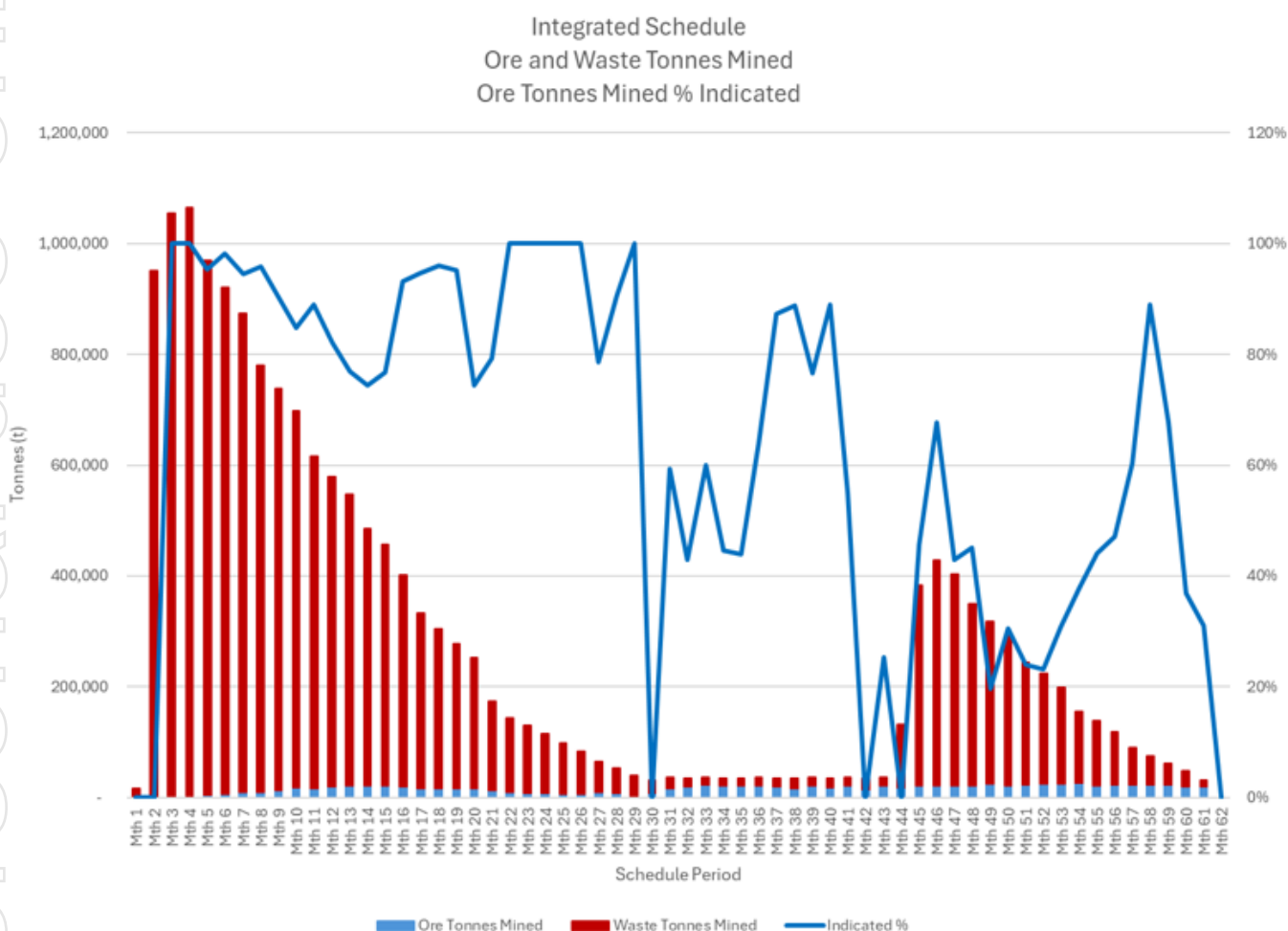
Figure 4, Ore and waste per month with % indicated category - transition to underground in month 27
