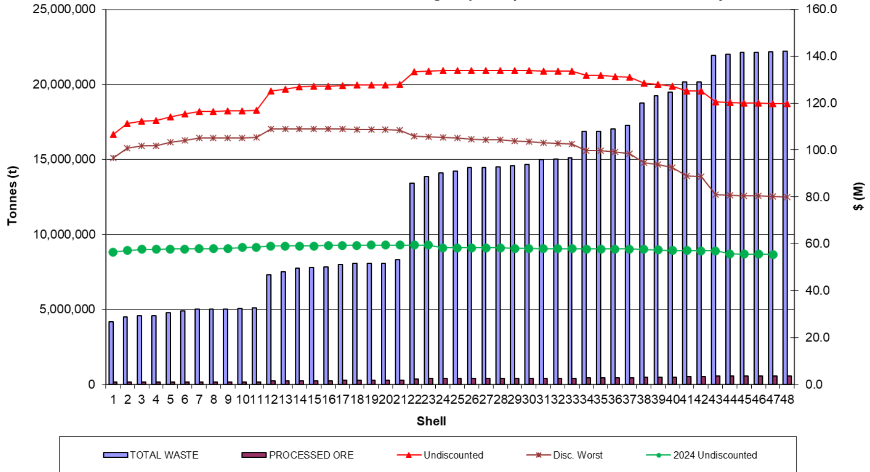
Figure 4-1 Kookynie Tonnage/Cash Flow Chart
