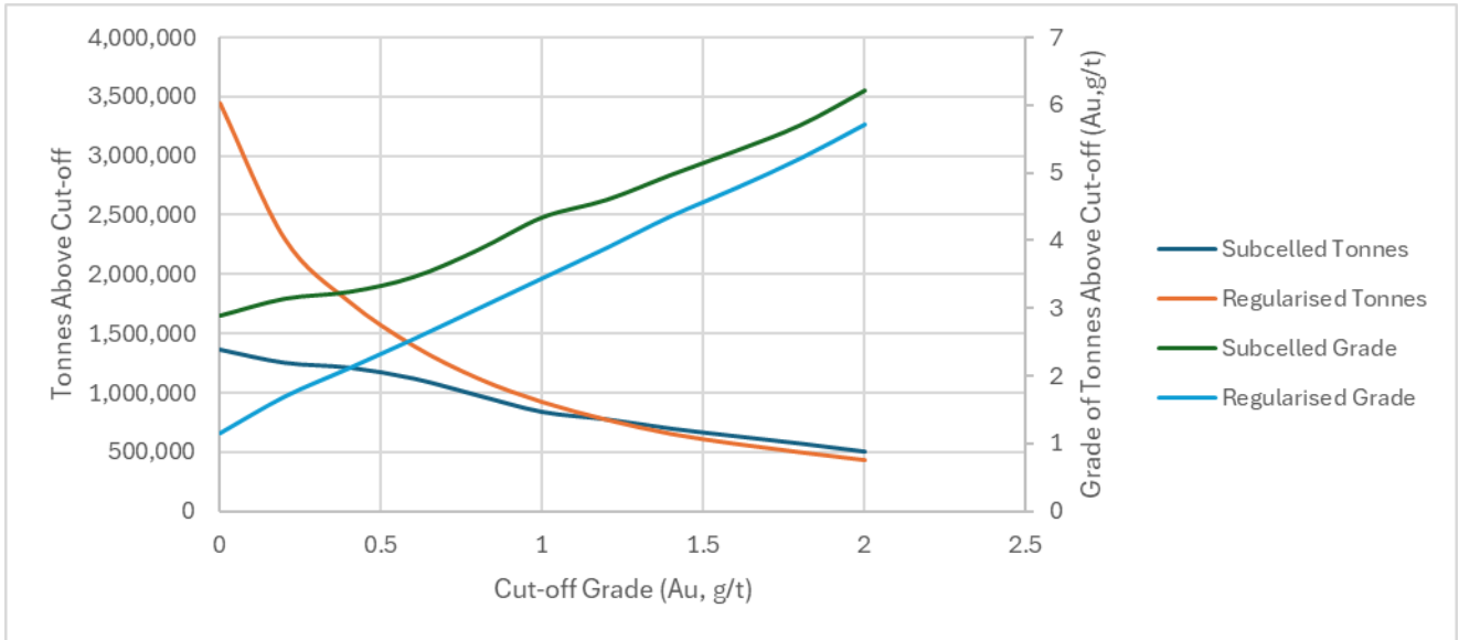
Figure 3-1 Grade-Tonnage Curve showing Resource and Mining (regularised) models
